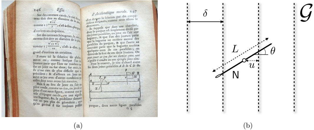
Figure 1: (a) Picture of [19, page 147] stating the initial formulation of Buffon’s needle problem (Courtesy of E. Kowalski’s blog http://blogs.ethz.ch/kowalski/2008/09/25/buffons-needle ). (b) Scheme of Buffon’s needle problem
