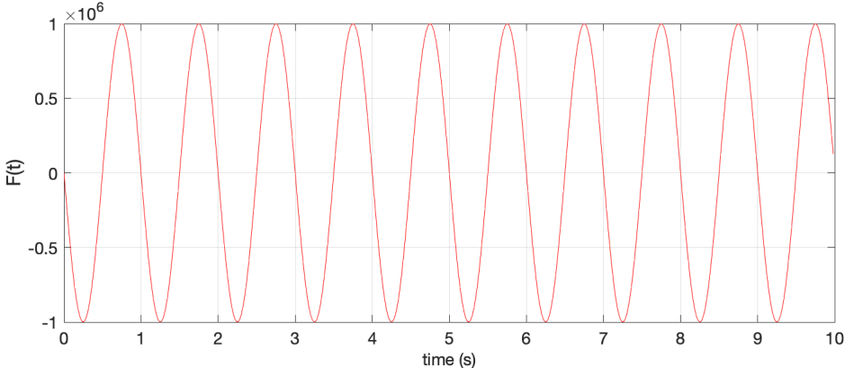
Figure 2. Harmonic loading.
