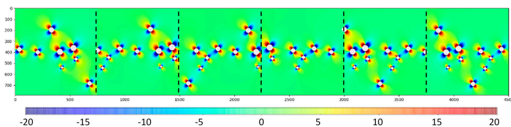
Figure 8. Fiber deviation map ( ^{\circ} ).
