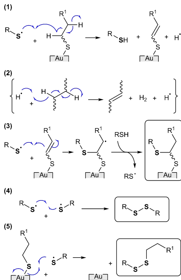
Scheme 1: Reaction mechanisms initiated by thiyl radical, RS^\cdot .
