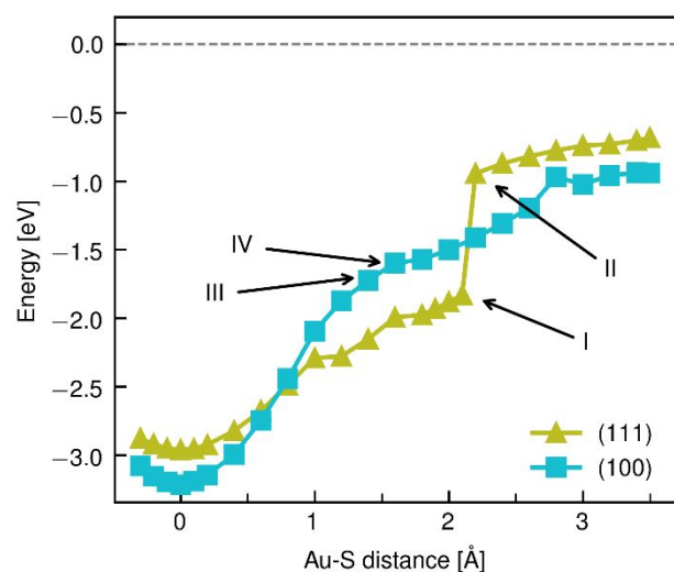
Figure 3: Left panel: Energy vs vertical distance between the S atom and the gold surface for both, (111) and (100) facets, at high coverage. The origin of the abscissa corresponds to the equilibrium Au-S distance. Right panel: snapshots of the local atomic configuration before and after the break of Au-S bonds for the pulled molecules on each Au surface. (I) and (III) correspond to the Au-S distance just before the bond break for the (111) and (100) surfaces, respectively. The gold ad-atom pulled is highlighted in orange. In (II) the detachment of a RS' is highlighted by the sulfur atom in green, while in (IV) the S-S bridge is remarked.
