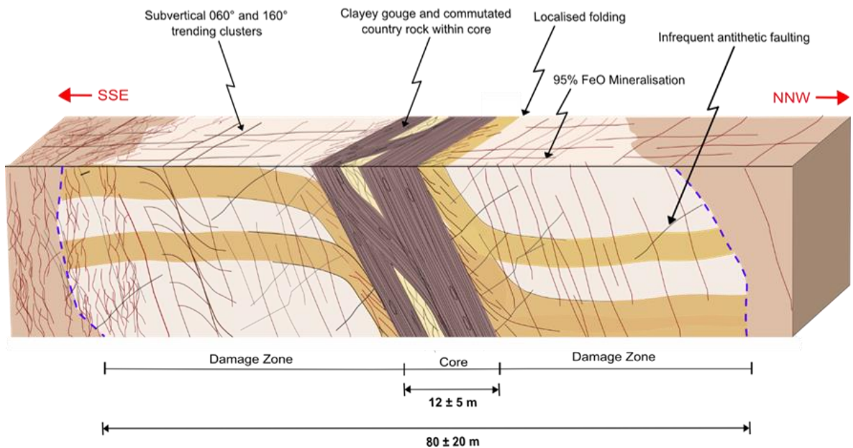
Figure 6: Schematic overview of the Dura Den and Maiden Rock Faults, showing the relative widths of the core and damage zone and fracture trends within these zones. The Dura Den fault can be characterised as having widespread fracturing in minimal mineralisation. Dominant subvertical fracturing suggests that along-fault fluid flow within the DDF would be enhanced, whilst normal faulting would accommodate across-fault flow. The Maiden Rock Fault is almost entirely mineralised with extensive clayey gouge in the fault core, rendering the fault a regional barrier to groundwater flow. The two faults can thus be respectively categorised as a ‘distributed conduit’ and ‘localised barrier’ (Caine, et al. , 1996).
