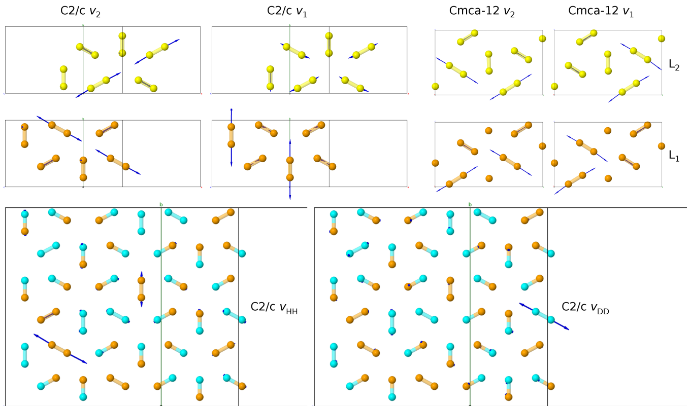
FIG. 1: Upper panels show the two most intense IR-active vibron modes at 250 GPa in pure hydrogen, assuming (a) C2/c and (b) Cmca-12 structures (24 atoms). The unit cells comprise two layers, shown separately for clarity ( L_1 - orange and L_2 - yellow). (c) Displacements corresponding to IR-active vibrons from C2/c cell (288 atoms) of disordered mixture at 250 GPa. Orange: H; cyan: D. Isotopic symmetry breaking means that all modes obtain some IR-activity. These highly localized vibron modes shown are representative examples for the spectrum generated by mixtures.
