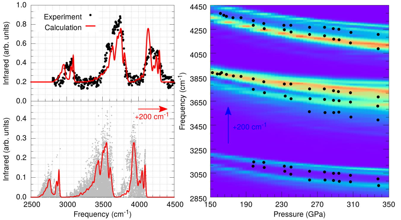
FIG. 4: Comparison of calculated IR in C2/c mixtures (see also Fig.3) to the recent raw experimental data [1]. We have removed the Gaussian fits made to the data by Dias et al since this approach is invalid to describe localised modes. Theoretically calculated spectra are systematically some 200\text{ cm}^{-1} softer than experimental spectra, due to a combination of errors including neglect of temperature, zero point effects in calculated pressure, calibration of the experimental pressure and choice of exchange-correlation functional [7, 10, 30]. (a) C2/c spectra at 300 GPa from 3000 randomized samples: gray dots are individual modes, red line is a histogram. (b) Comparison of the calculations to the digitized experimental data at 307 GPa [1, 31]. (c) Color map showing the calculated pressure dependence of the IR intensity compared to the equivalent experimental data [1].
