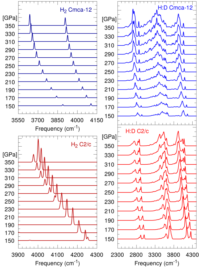
FIG. 3: Stacked plot of simulated vibronic infrared signal at different pressures (shown on y-axis) for the two candidate structures C2/c and Cmca-12 . Intensities are calculated so spectra at different pressure points are comparable. On the left pure hydrogen as (a) Cmca-12 (b) C2/c . Normal-mode linewidths narrower than experimental resolution[17] are chosen to emphasize the impossibility of resolving the two C2/c modes below 230 GPa. On the right we show the data for 50:50 hydrogen-deuterium mixtures (c) Cmca-12 (d) C2/c . Comparison in Fig4 (and SM) shows that C2/c is a better candidate than Cmca-12 . At low pressures C2/c has six distinct peaks, two for each molecular type ( \text{H}_2 , \text{HD} , \text{D}_2 ). The two peaks per molecule type here are not connected to the distinct peaks in the pure hydrogen spectra, but rather a signature of local molecular environments. This splitting is an indirect indication of mode localization, which confers some IR activity to all modes [30].
