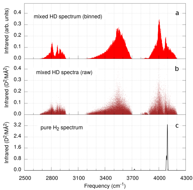
FIG. 2: Method used to calculate spectra in mixtures at 250 GPa from 288 atom calculations, explained in detail in SM[27]. (a) mixture data binned up in a histogram for comparison with experiment. (b) dot for the intensity of each of 144000 localized modes generated from 1000 random samples of hydrogen-deuterium mixtures. (c) IR spectrum of pure hydrogen C2/c .
