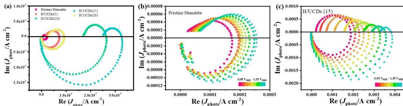
Fig. 6. IMPS plots for pristine hematite and H/UCDs photoelectrodes.
