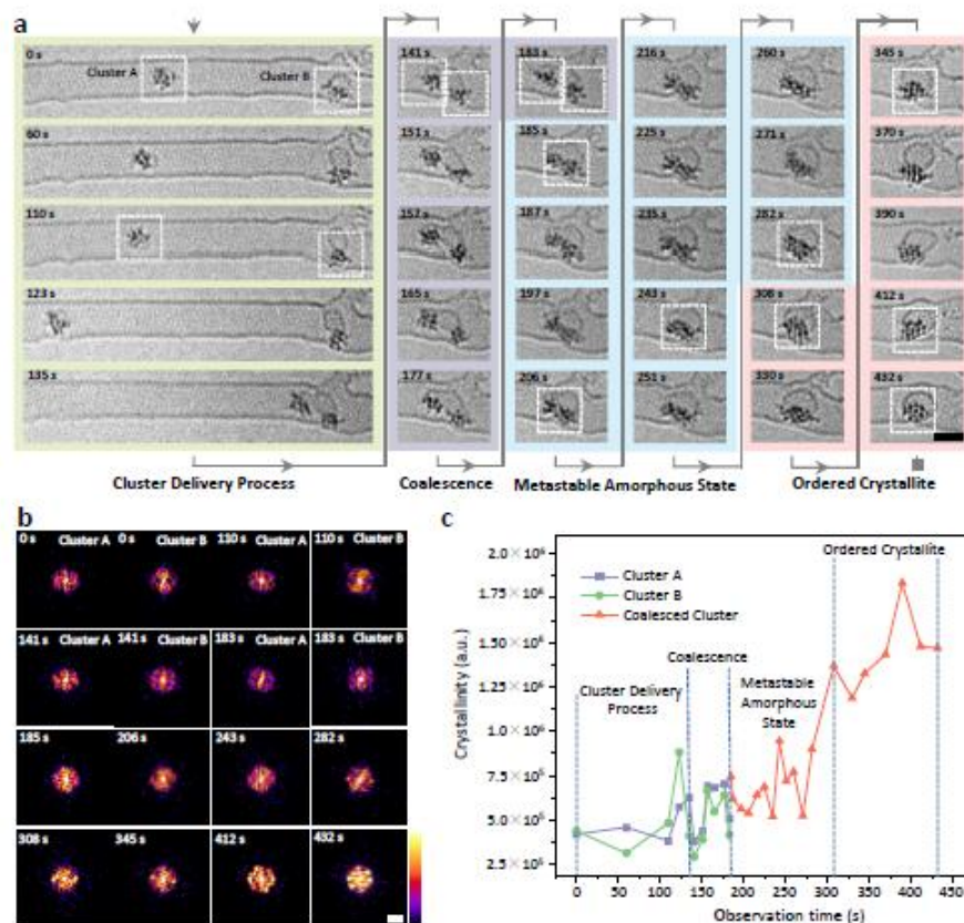
1 2 Figure 5 | E-beam stimulated nucleation of a Re crystallite by coalescing two amorphous 3 sub-nano Re clusters. a , Time-series AC-HRTEM images showing the four key stages of Re 4 crystallite nucleation starting with two amorphous sub-nm Re clusters (Supplementary Video 3). 5 From 0 s to 135 s, one amorphous cluster located at the left of the SWNT translates and attaches 6 to another amorphous cluster located at the right of the SWNT, which is the first stage of Re 7 nucleation, ‘Cluster Delivery Process’. From 141 s to 183 s, the two clusters contact each other 8 and then coalesce into one amorphous cluster, which is the second stage: ‘Coalescence’. The 9 coalesced amorphous cluster ceaselessly changes its structure from 185 s to 282 s, ‘Metastable 10 Amorphous State’ stage. At 308 s, a crystallite is formed and keeps on restructuring for a further 11 124 seconds, ‘Ordered Crystallite’ stage; scale bar, 1 nm. b , FFT patterns of the corresponding 12 areas framed by white dotted boxes in a analyzing the periodic structural information of Re
