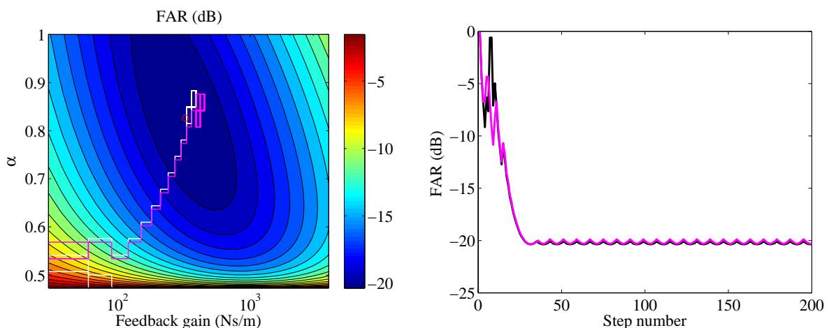
Figure 8: The convergence behaviour of the auto-adaptive controller with increased and adjusted increments, and with decreased averaging time per step.
