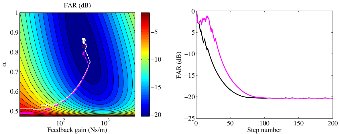
Figure 4: The convergence behaviour of the auto-adaptive controller
