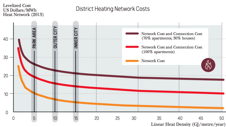
Figure 16. An example of network costs for DH systems [16]
