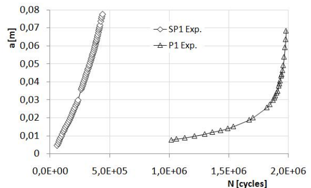
Slika 3. Životni vijek uzoraka P1 i SP1–eksperiment Figure 3. Experimental fatigue lives for P1 and SP1 specimens
