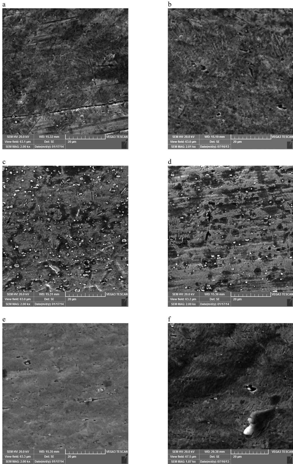
Figure 1. Scanning electron microscope images (2000× magnification) of as-received (left column) and after electrochemical testing (right column) of nickel-titanium (NiTi) wire samples. (a, b) Uncoated NiTi. (c, d) Rhodium-coated NiTi. (e, f) Nitrified NiTi.
