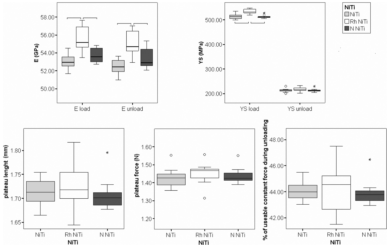
Figure 2. Loading and unloading elastic modulus ( E ), yield strength ( YS ), and parameters of unloading slope for nickel-titanium (NiTi) wires (uncoated [NiTi], nitrided [N NiTi], and rhodium-coated [Rh NiTi] wires). Statistically significant differences are marked with horizontal bars ( P < .05 ).
