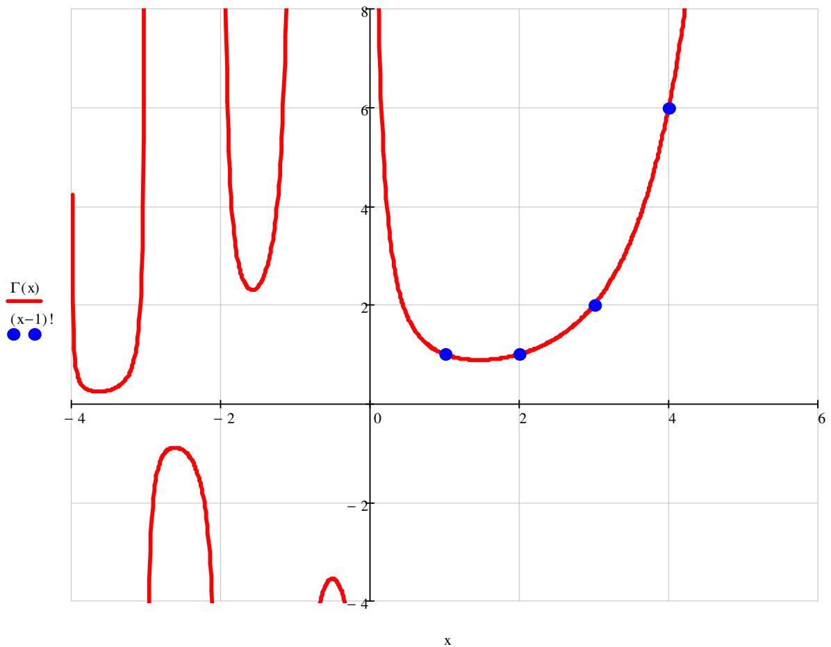
Fig. 1. Gamma function and the approximation to the factorial function
