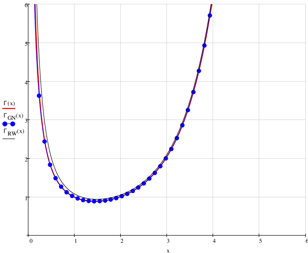
Fig. 2. Comparison of approximate Gamma function formulations with the complete Gamma function
