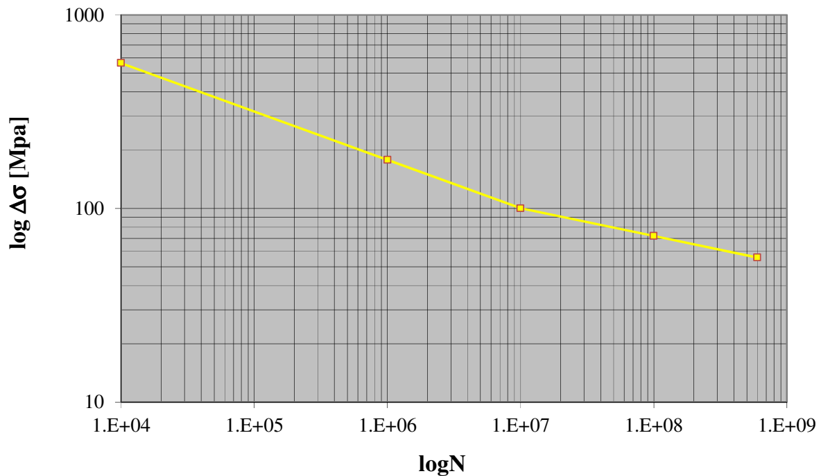
Fig. 3. S-N curve, Class B
