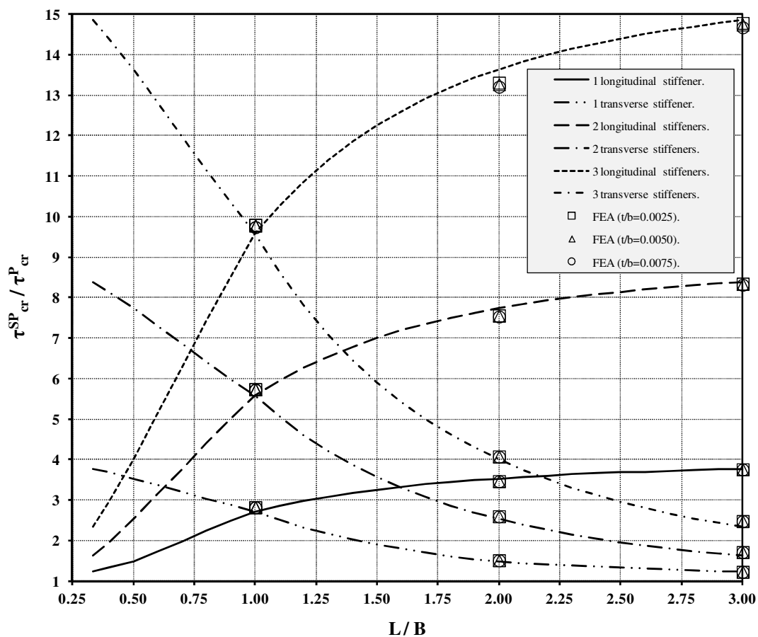
Fig. 2. Maximum increase in the elastic shear buckling capacity attainable by the plate stiffening.
