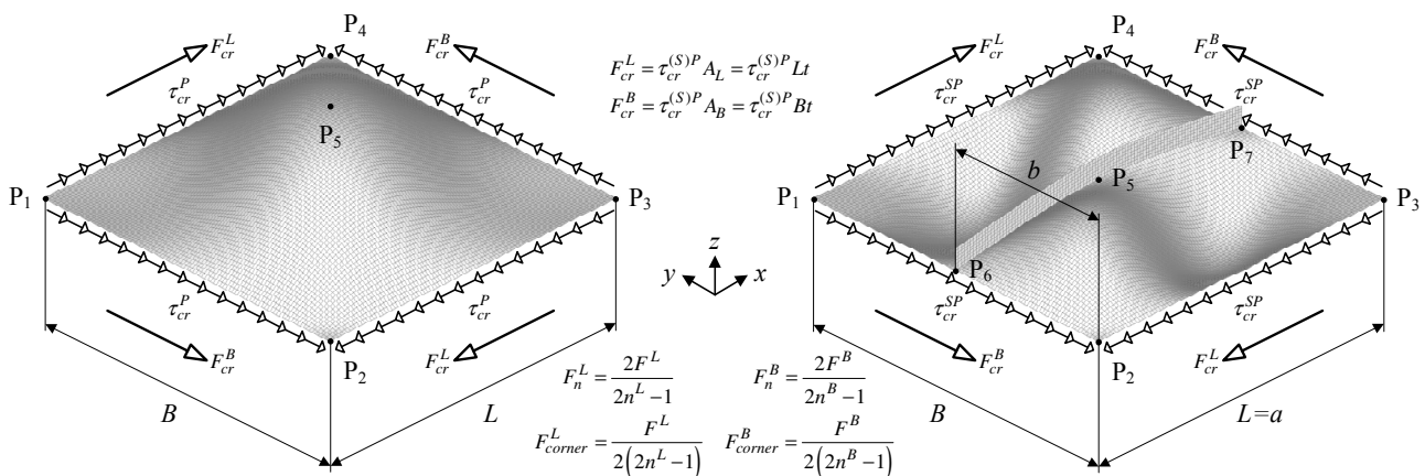
Fig. 1. Elastic shear buckling of the simply supported (un)stiffened plate.
