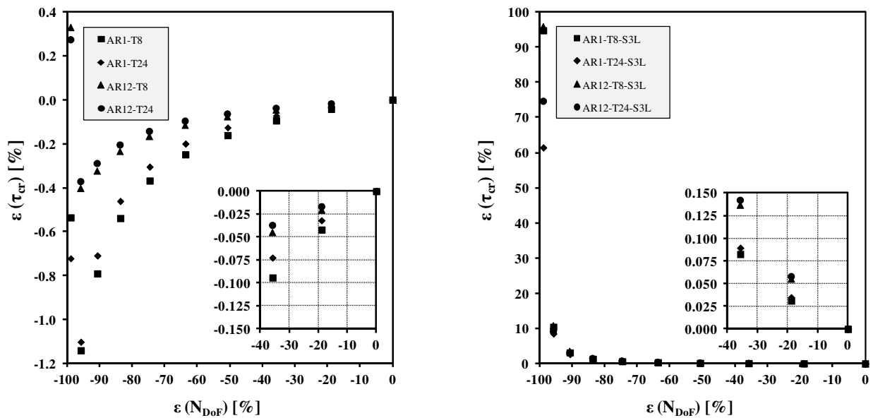
Fig. 3. Results of the mesh convergence study.
