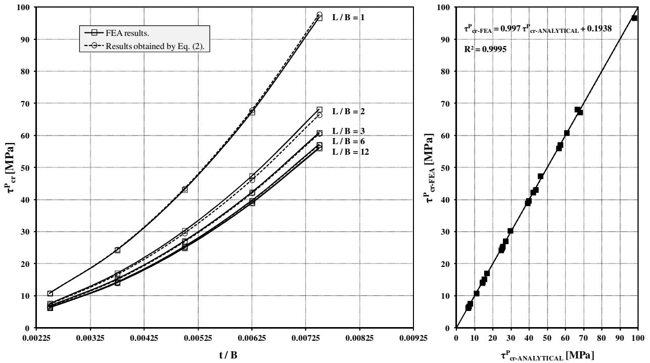
Fig. 4. Unstiffened plate results obtained by FEM analyses and Eq. (2).
