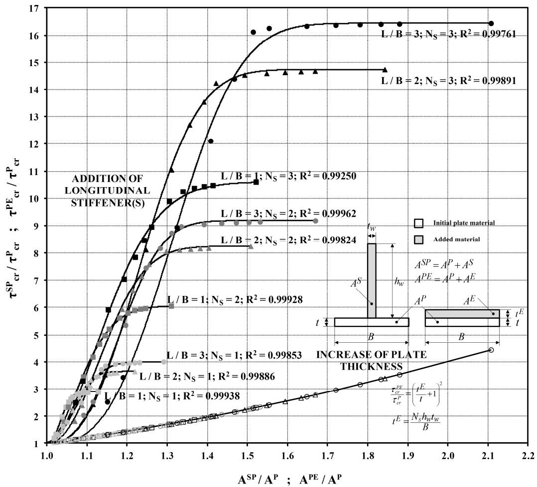
Fig. 5. Results obtained by longitudinal stiffening and increase of plate thickness.
