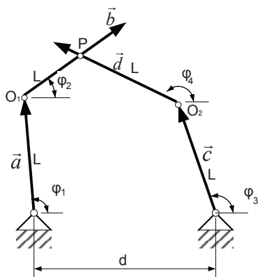
Figure 7. Analysis of intersection P between the top links of the robots
