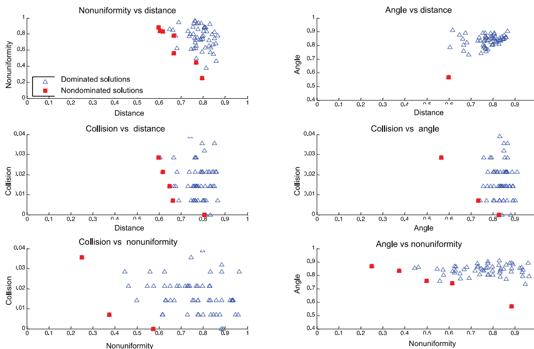
Figure 5. Pareto fronts in an early phase of evolution ( G=30 ) for various pairs of evaluation criteria
