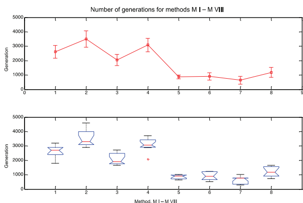
Figure 6. Impact of the modified co-evolution on the convergence speed
