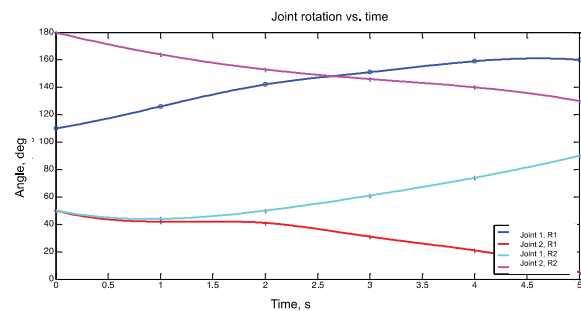
Figure 9. Interpolated joint rotation values for discrete values obtained by the co-evolutionary algorithm
