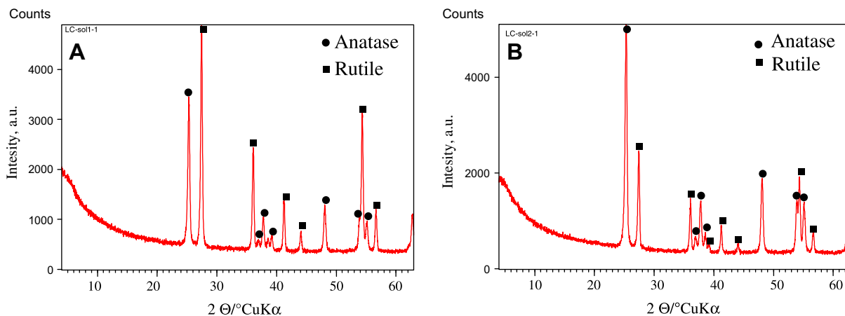
Fig. 2. XRD patterns of the \text{TiO}_2 powder prepared (A) without the addition of PEG to the initial sol 1 and (B) with the addition of PEG to the initial sol 2.
