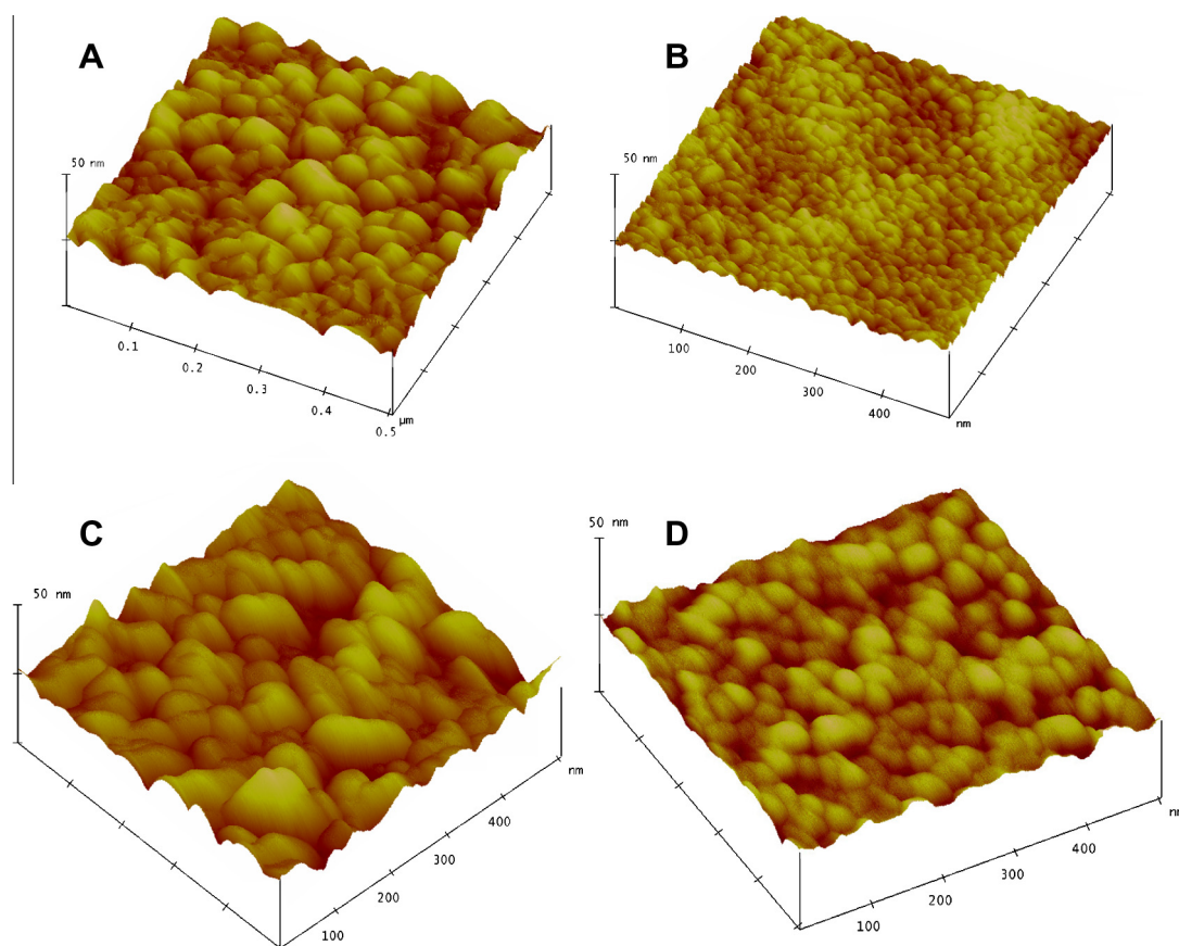
Fig. 3. Three dimensional AFM micrograph of deposited \text{TiO}_2 films: (A) \text{TiO}_2 film 1 with one layer, (B) \text{TiO}_2 film 1 with three layers, (C) \text{TiO}_2 film 2 with one layer and (D) \text{TiO}_2 film 2 with three layers. All images are taken in 500 \text{ nm} \times 500 \text{ nm} area. Vertical scale in all images is 50 nm. Film 1 (obtained from sol without PEG) and film 2 (obtained from sol with PEG).
