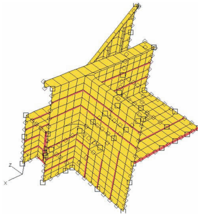
Figure 5 Fine mesh model of the aft hatch corner (squares represent imposed displacements from the coarse mesh model)
