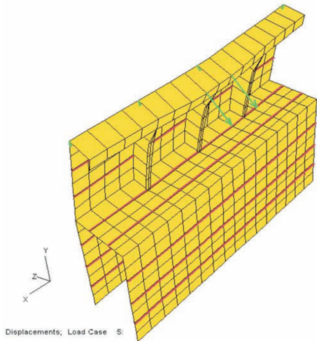
Figure 7 Concentrated forces and deformations of the fine mesh hatch coaming model
