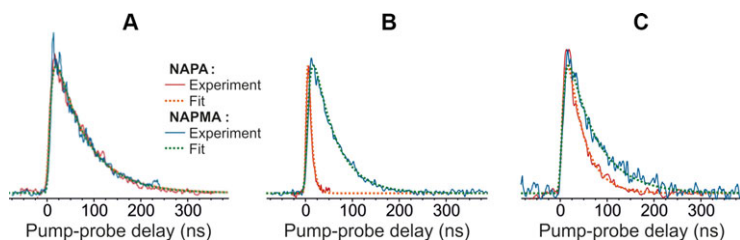
Figure 2.4: Pump-probe nanosecond signals obtained after pumping the origin transition of conformers A, B and C of NAPMA (blue) and NAPA (red). Lifetime values of best fits (dotted lines) are given in Table 2.1. Figure adapted from reference [33].
