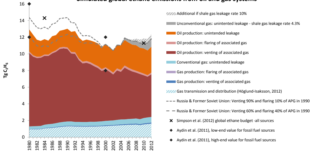
Simulated global ethane emissions from oil and gas systems
