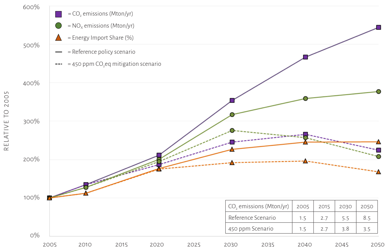
Figure 1: Projections of CO 2 emissions, NO x emissions, and primary energy import share for India
