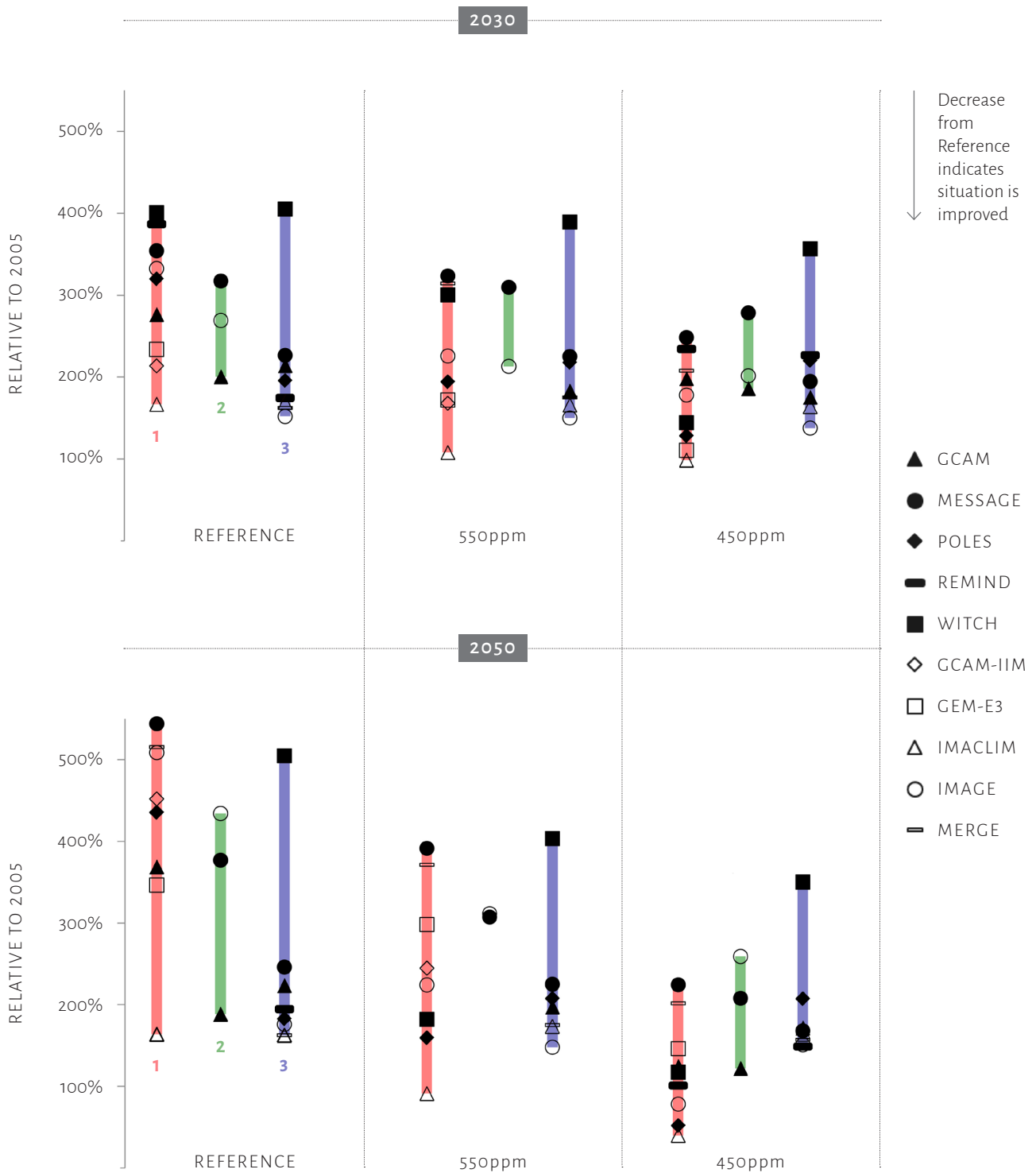
Figure 2: Multiple Model Results for Indian CO 2 emissions, NO x emissions, and primary energy import share, relative to 2005 levels.
