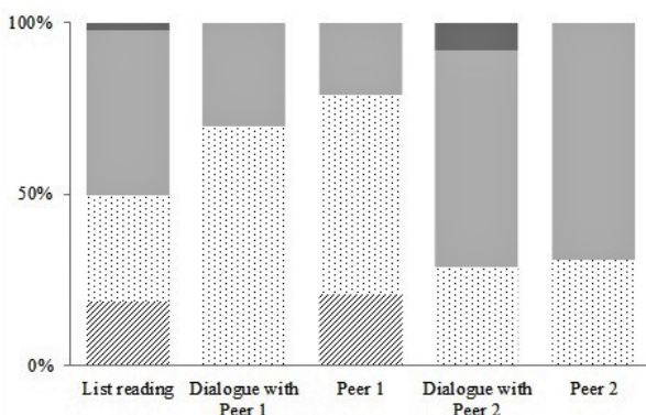
Figure 6. Proportion of R variants produced for geminate /rr/ by the target speaker and his interlocutors when speaking dialect. Striped bars correspond to taps, dotted to trills, dark grey to approximants, light grey to fricatives.
