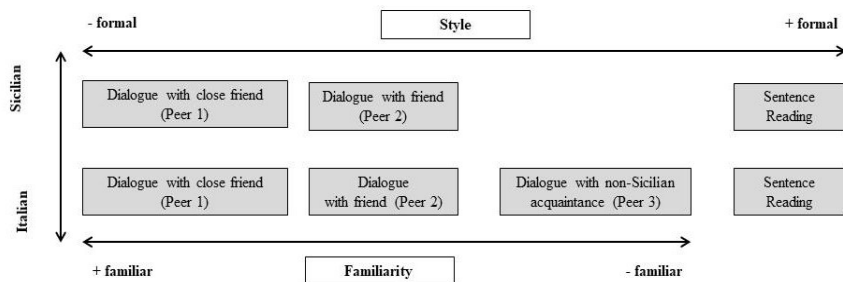
Fig. 1. Language variety, style and familiarity co-variation in the SoPhISM corpus.
