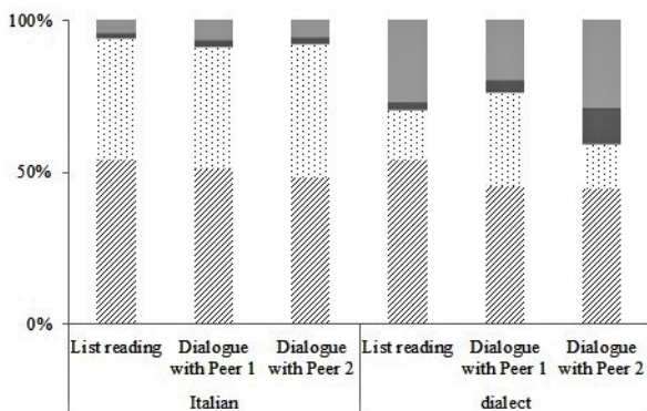
Fig. 2. Proportion of R variants produced by the target speaker in each speech task as a function of language and (for dialogues) interlocutor. Intervocalic singletons and geminates conflated. Striped bars correspond to taps, dotted to trills, dark grey to approximants, light grey to fricatives.
