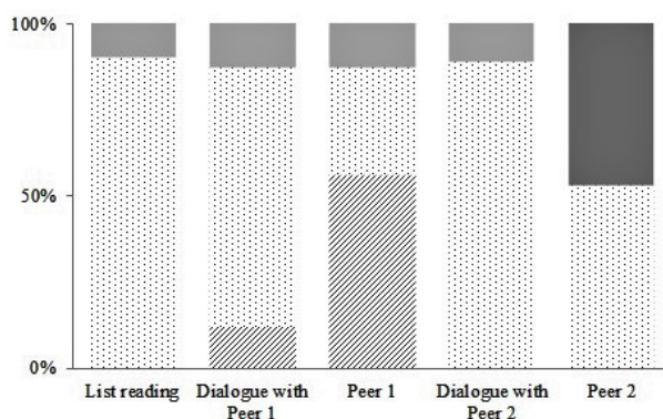
Figure 4. Proportion of R variants produced for geminate /rr/ by the target speaker and his interlocutors when speaking Italian. Striped bars correspond to taps, dotted to trills, dark grey to approximants, light grey to fricatives.
