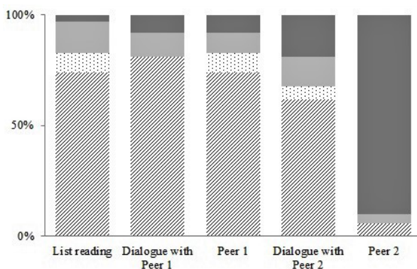
Figure 5. Proportion of R variants produced for singleton /r/ by the target speaker and his interlocutors when speaking dialect. Striped bars correspond to taps, dotted to trills, dark grey to approximants, light grey to fricatives.
