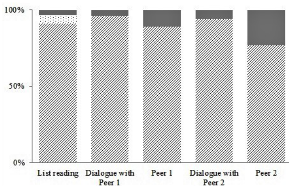
Figure 3. Proportion of R variants produced for singleton /r/ by the target speaker and his interlocutors when speaking Italian. Striped bars correspond to taps, dotted to trills, dark grey to approximants, light grey to fricatives.
