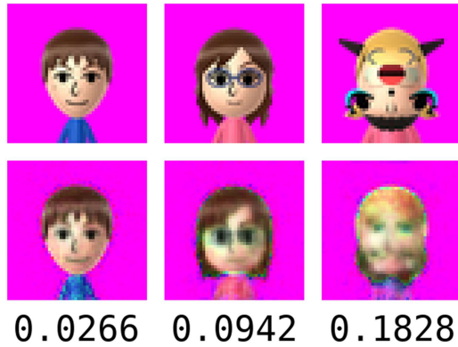
Fig. 2. Low-novelty, medium-novelty, and high-novelty Miis (top) along with their reconstructions by our network (bottom) and corresponding prenormalization novelty values (units are per-pixel-channel root-mean-squared error of each reconstruction in 255-value HSL). The left Mii is very close to the default male Mii, while the center Mii is more novel in part because there are relatively few female-presenting avatars in the dataset. Note how the network tries (and fails) to reconstruct the high-novelty Mii from more typical facial features. The images are shown at 48 \times 48 pixels, the same resolution the network uses.
