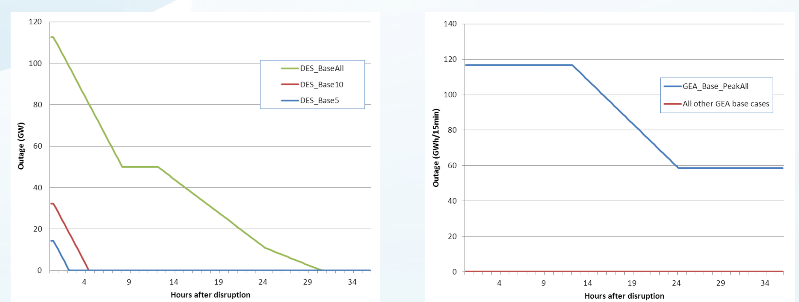
Figure 2: Potential outage size and duration for the simultaneous disabling of 5, 10 and all (33 and 83, respectively) chokepoints for Desertec (left) and GEA (right). Source: Lilliestam (in review)
