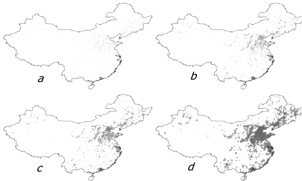
Fig. 2: Results showing the development of night-time lights in China. a: initial (1995/1996) state, b: total increase by factor 5, c: total increase by factor 10 d: total increase by factor 40.
