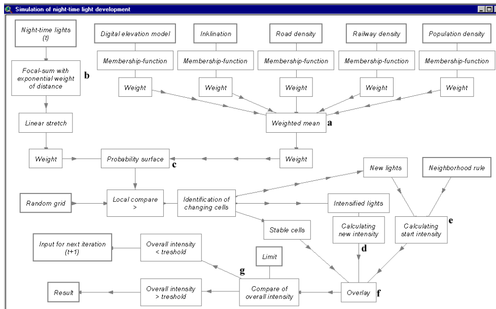
Fig. 1: MapModel to simulate the spatial and temporal development of night-time lights.
