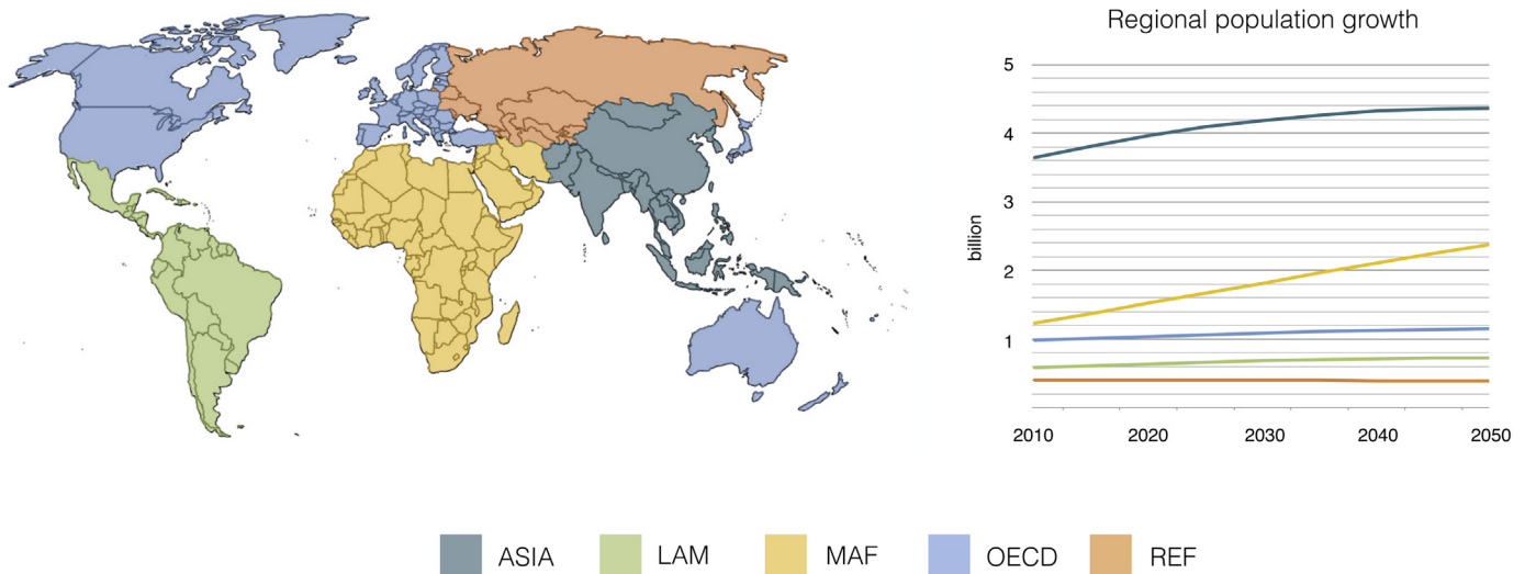
Fig. 2. SSP world regions and population growth as projected for each region. The map displays the five world regions Asia (ASIA), Latin America (LAM), MAF (Middle East and Africa), OECD countries (OECD) and the countries from reforming economies of Eastern Europe and the former Soviet Union (REF). The graph on the right presents the projected population growth for each world region until 2050.
