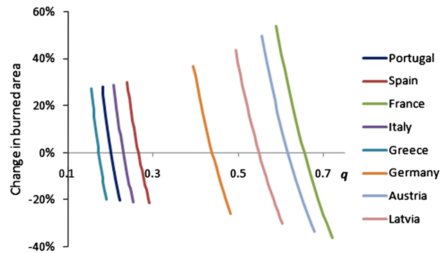
Fig. 4 Sensitivity analysis of suppression efficiency for the SFM model calibrated using GFED data for years 2000–2008. Changes in burned areas per country are in percents relative to burned area corresponding to calibrated value of q (values of q vary within \pm 10\% range)
