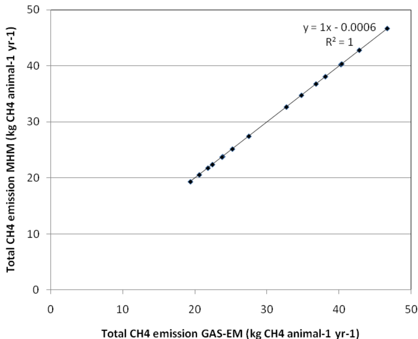
Figure 4. Total CH 4 emission (storage+grazing) for dairy cows in liquid manure systems in Germany: results of MHM vs. GAS-EM.
