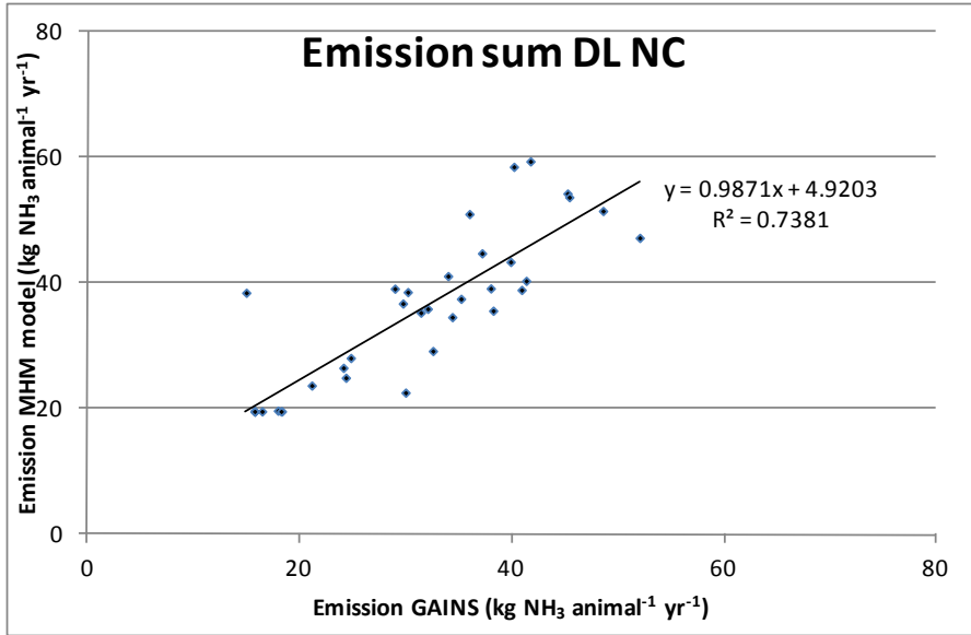
Figure 9. Total emission factors of NH 3 for dairy cows in a liquid manure system without any abatement (housing+storage+application+grazing): results of MHM vs. GAINS. Data points represent individual countries.
