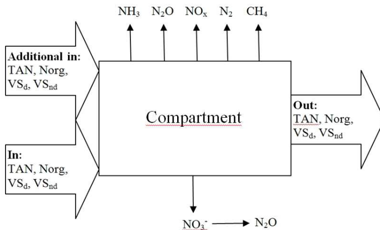
Figure 2. Set-up of one compartment, with input and output and emissions. The input called “In” comes from a previous step in the manure handling model, whereas the input called “Additional in” is fresh input (either bedding material or organic waste). The \text{NO}_3^- emission originating from leaching of manure heaps and runoff gives rise to \text{N}_2\text{O} emission.
