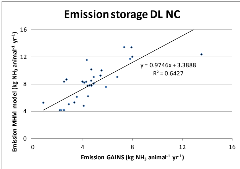
Figure 6. Emission factors of NH 3 from storage for dairy cows in a liquid manure system without any abatement: results of MHM vs. GAINS. Data points represent individual countries.
