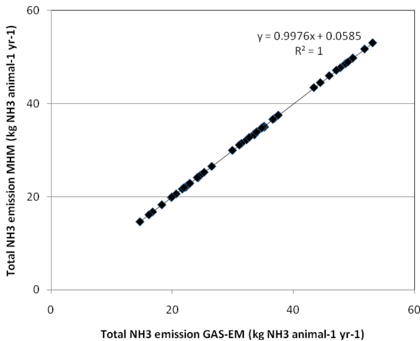
Figure 3. Total NH 3 emission (housing+storage+application+grazing) for dairy cows in liquid manure systems in Germany: results of MHM vs. GAS-EM.
