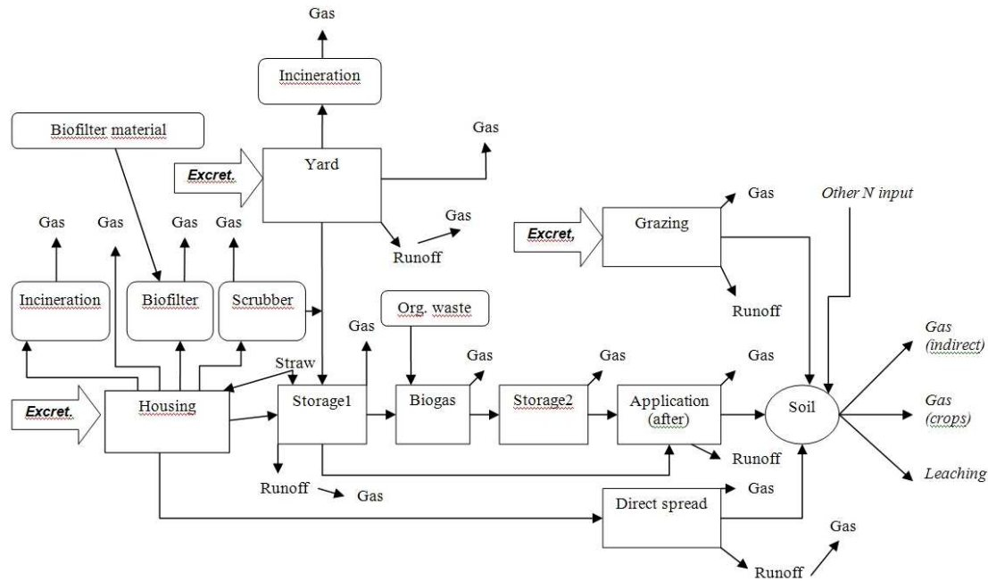
Figure 1. Set-up of the manure handling model. Excretion may include other animal material further processed. The figure indicates the maximum number of processes that can be described in the model. In practice fewer processes will be modeled. This situation can be handled by either setting some parameters to zero or by using by-pass switches. The processes at the right side of the figure described in italic font occur outside of the model. The excreted manure can enter the model in three different places: housing, yard and during grazing. The rectangles indicate compartments, where manure is input and output. The rounded rectangles indicate compartments, where this is not the case.
