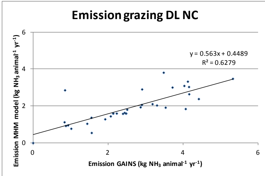
Figure 8. Emission factors of NH 3 during grazing for dairy cows without any abatement: results of MHM vs. GAINS. Data points represent individual countries.
