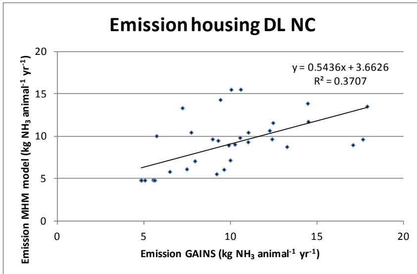
Figure 5. Emission factors of NH 3 from housing for dairy cows in a liquid manure system without any abatement: results of MHM vs. GAINS. Data points represent individual countries.
