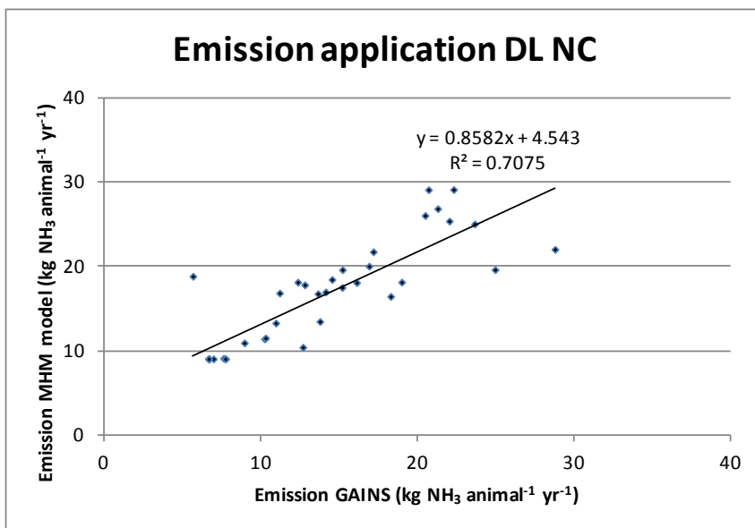
Figure 7. Emission factors of NH 3 after application housing for dairy cows in a liquid manure system without any abatement: results of MHM vs. GAINS. Data points represent individual countries.
