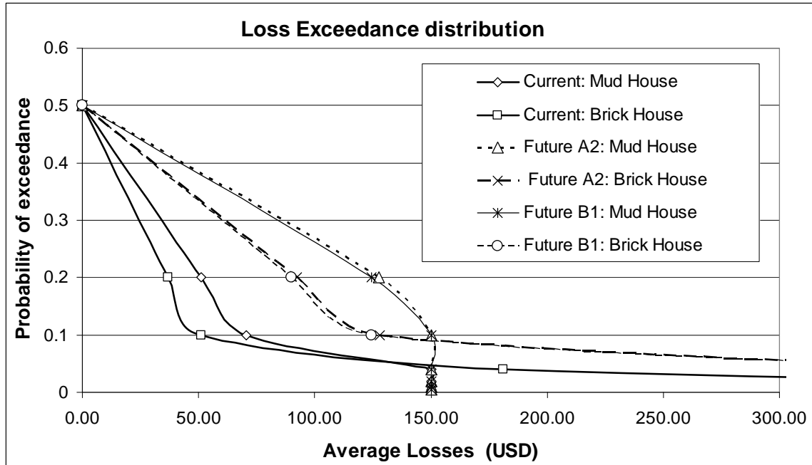
FIGURE 9: LOSS EXCEEDANCE PROBABILITIES TAKING ACCOUNT OF CLIMATE CHANGE AT 2030
