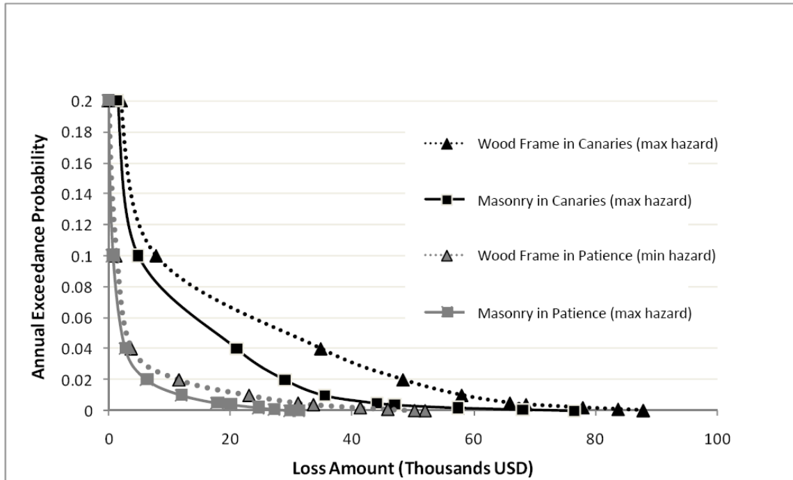
FIGURE 3: EP CURVES WITH NO DRR - HURRICANE RISK IN ST. LUCIA
