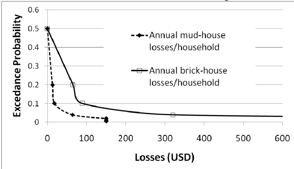
FIGURE 7: FLOOD RISK WITHIN THE ROHINI RIVER BASIN IN INDIA - LOSS EXCEEDANCE FUNCTION FOR BRICK AND MUD CONSTRUCTED HOUSES
