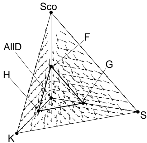
Figure 4: The system with AIIID and 3 types of discriminators. AIIIC is not involved. The surface FGH given by x_2 = 1 - c/\bar{\epsilon}b consists of unstable fixed points, where x_2 is the frequency of AIIID . Depending on which side of that surface they start from, orbits converge either to the segment S-K or to the segment AIIID-F .
