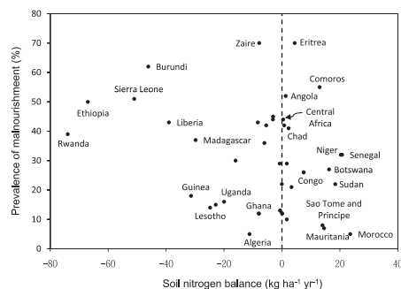
Fig. 2. BAL _{\text{soil}} and prevalence of malnourishment in Africa in 2000. The prevalence of undernourishment in the total population (%) is obtained from the FAO (20). Data for the period 2000–2002 are used. BAL _{\text{soil}} is estimated in this study.
