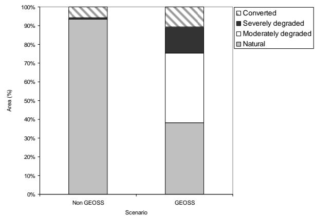
Figure 1: Land cover categories and percentage coverage based on GEOSS and non GEOSS scenario databases for the Little Karoo of South Africa.
