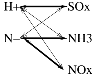
Figure 6: Illustration of compatibilities for transfer coefficients.
