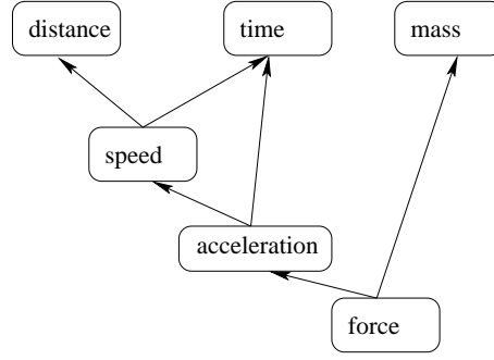
Figure 1: Example of gPDs. A directed edge from gPD_i to gPD_j signifies that gPD_j appears in gPD_i 's definition.
