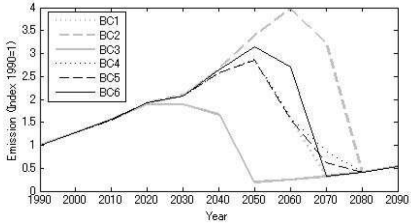
Figure 8. Different carbon emission paths.
