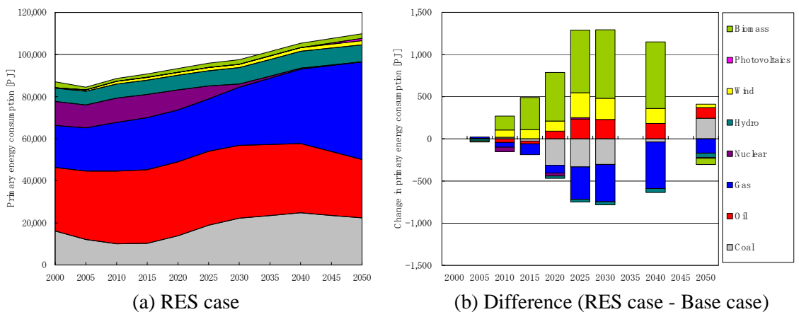
Figure 5.32 Primary energy consumption (EU30)
