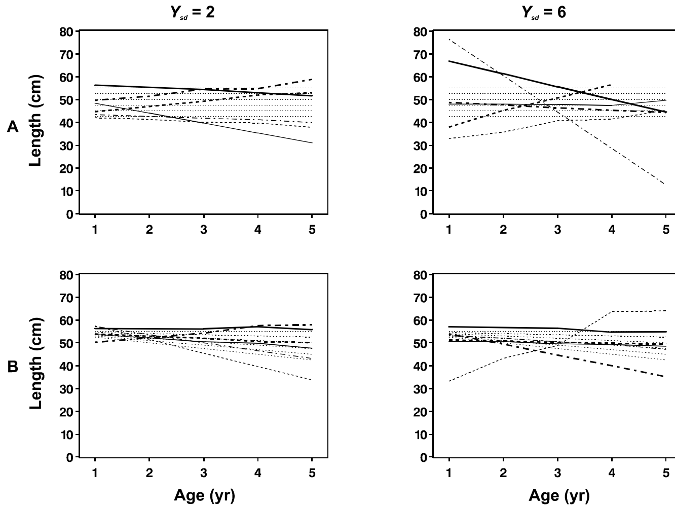
Figure 7. Graphic example of robustness tests. (A) For the first test (no age effect), theoretical reaction norms are horizontal and shift vertically. (B) For the second test (age effect), reaction norms of the successive cohort are more and more tilted clockwise. Five cases, corresponding to an increase in the year effect ( Y_{sd} ) on the reaction norm midpoints have been considered, and two cases are displayed here. Because the reaction norms of 30 cohorts cannot be displayed on the same figure, the reaction norms of 6 evenly spaced cohorts are displayed. Thin dotted lines, theoretical reaction norms ———, cohort 0; — · — · —, cohort 5; ·····, cohort 10; ———, cohort 15; - · - ·, cohort 20; ·····, cohort 25.
