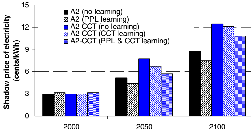
Figure 6: Shadow prices of electricity.
