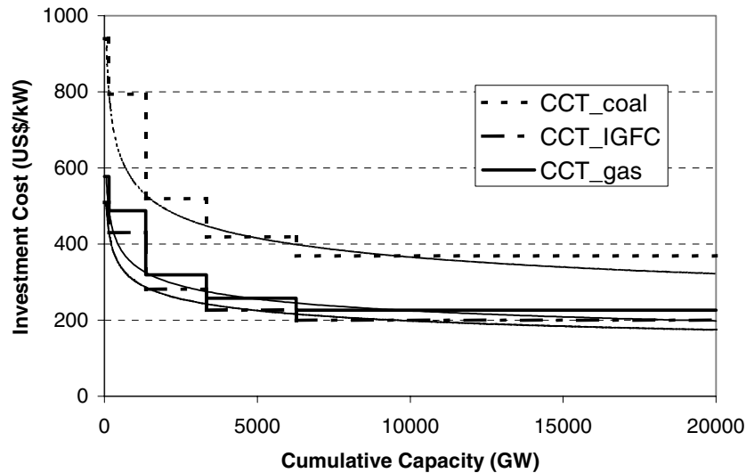
Figure 2: Learning curves assumed in this exercise for the carbon-capture clusters considered in the power sector. The step-wise approximation and the original non-linear curve are presented.
