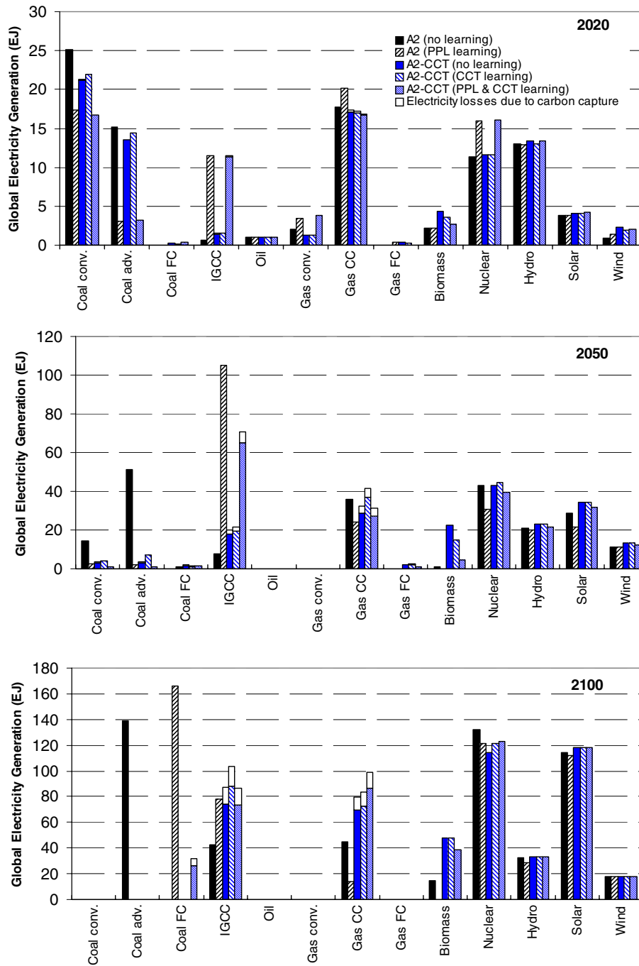
Figure 4: Global electricity generation for the A2 and A2-CCT scenarios in the years 2020, 2050 and 2100. For the A2-CCT cases, electricity losses due to the carbon capture process are shown as white bars.
