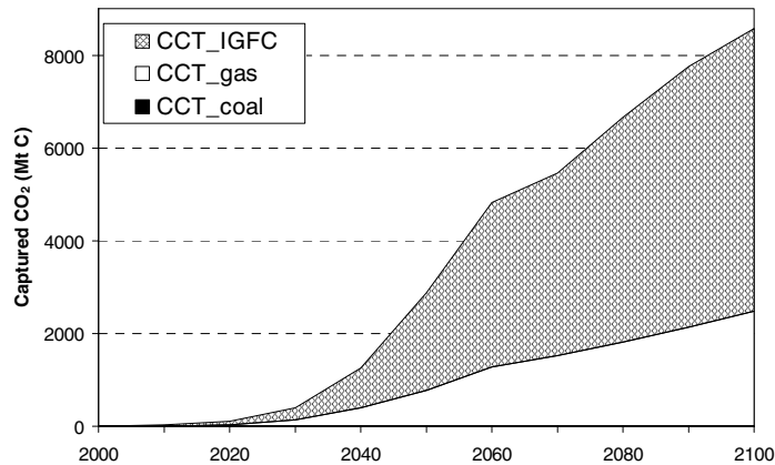
Figure 11: Captured CO 2 along the time horizon in the A2-CCT (PPL & CCT Learning) scenario. The contributions of the three CCT clusters are distinguished.
