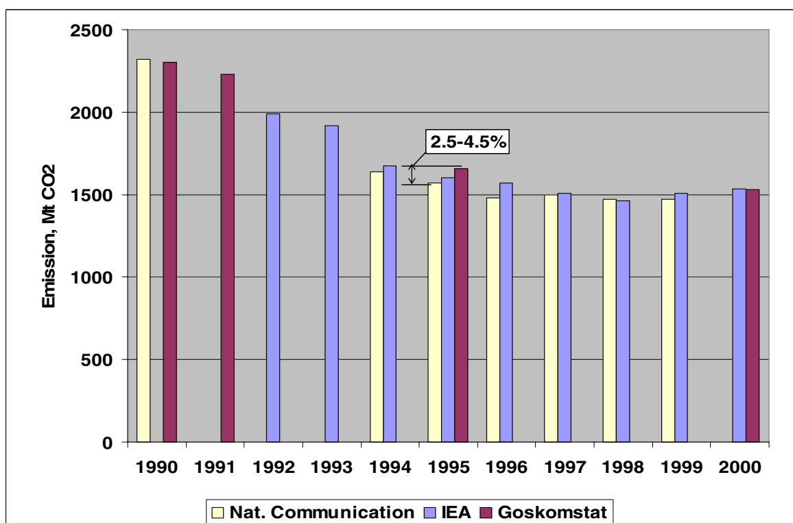
Figure 7: Results of Reference Approach inventory of CO 2 emissions from the Russian energy sector.
