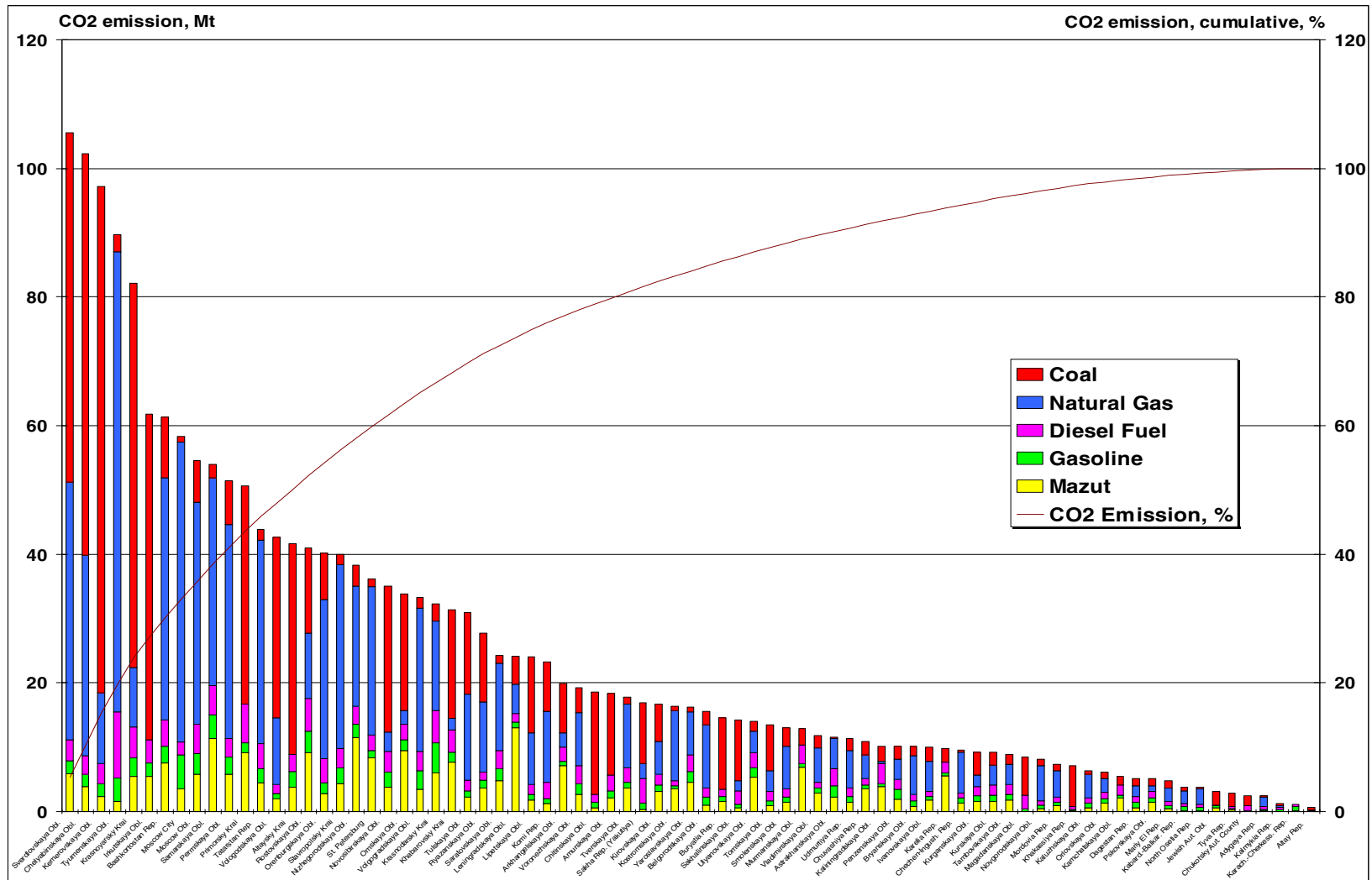
Figure 6: Regional structure of CO 2 emissions in the Russian Federation in 1990.
