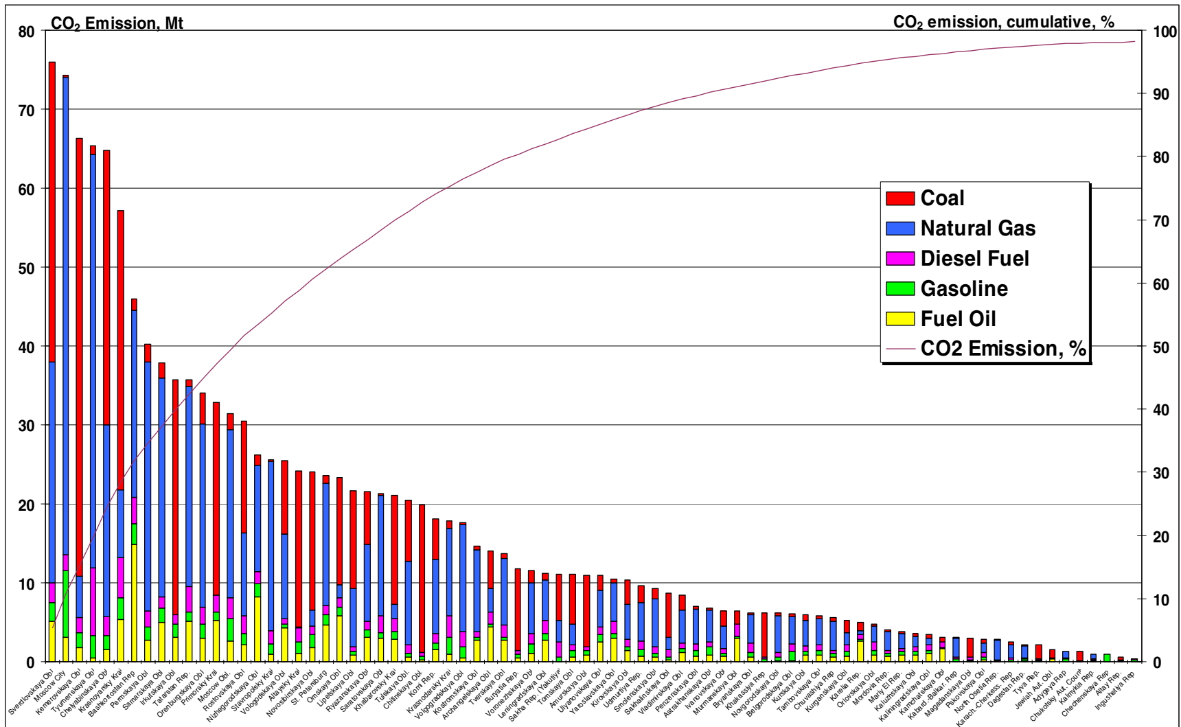
Figure 4: Regional structure of CO 2 emissions in the Russian Federation in 1997.
