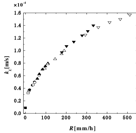
Figure 9. Relationship between R and k_L ; solid square: no rain, open square: d_n=0.40 \text{mm} , solid circle: d_n=0.45 \text{mm} , open circle: d_n=0.50 \text{mm} , solid triangle: d_n=0.55 \text{mm} , open triangle: d_n=0.65 \text{mm} , down pointing solid triangle: d_n=0.70 \text{mm} , down pointing open triangle: d_n=0.80 \text{mm} .
