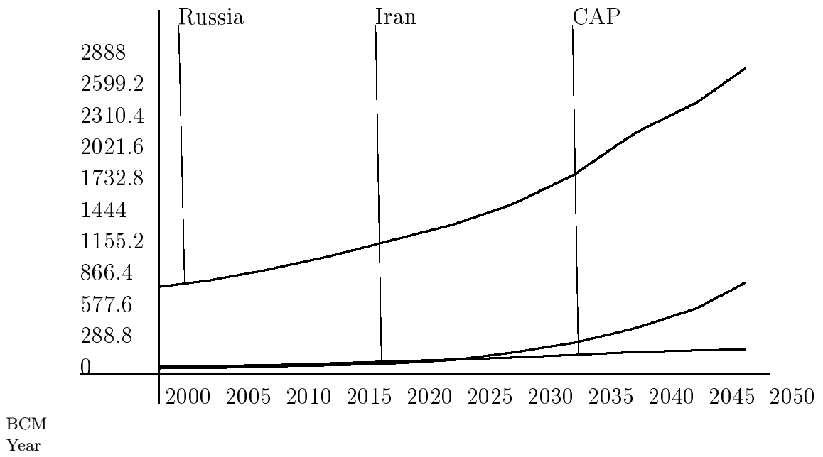
Figure 2: Exogenous gas demand functions.
