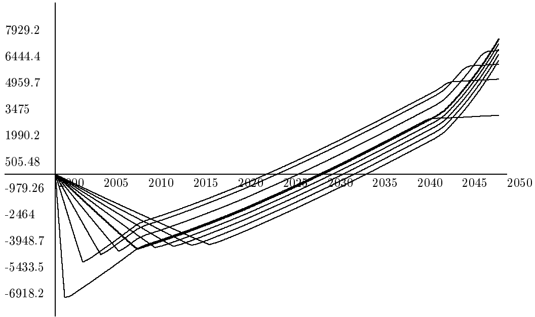
Figure 12: Case A, Scenario 2: Net present values of “Blue Stream” depending on delivery time.
