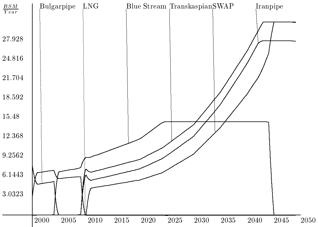
Figure 19: Case A, Scenario 5: Supply by competitive pipelines under optimization of “Blue Stream” maximal capacity.
