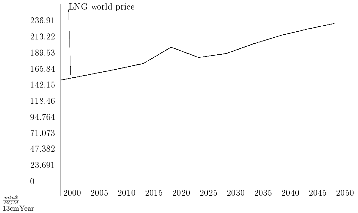
Figure 3: Dynamics of LNG world market price.
