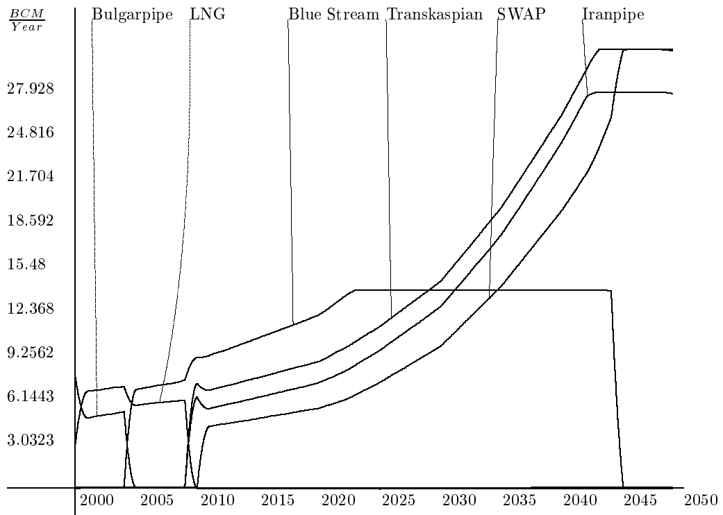
Figure 16: Case A, Scenario 4: Gas deliveries of competitive pipelines.
