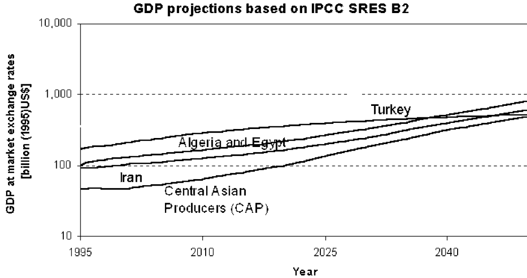
Figure 5: GDP projection for the period 1998-2050.
