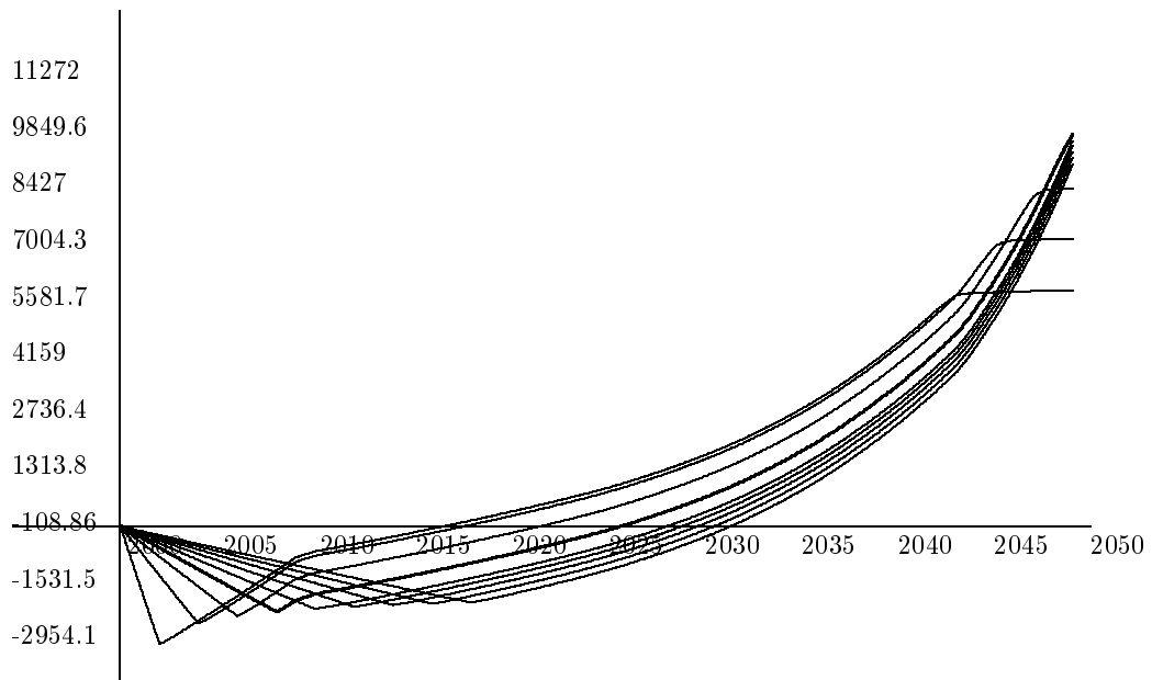
Figure 15: Case A, Scenario 3: Net present values of “Transcaspian” depending on delivery time.
