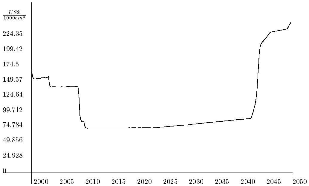
Figure 11: Case A, Scenario 1: Gas price.
