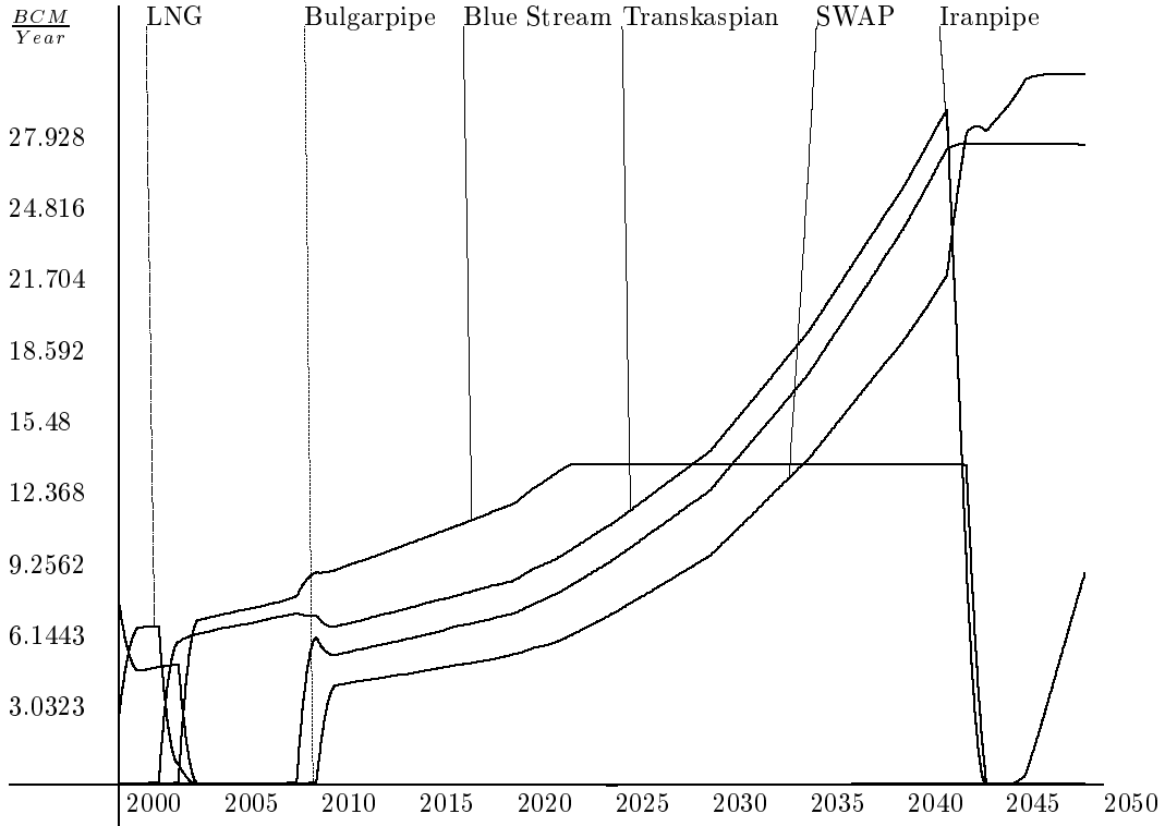
Figure 9: Case A, Scenario 1: Gas supply (bcm/year).
