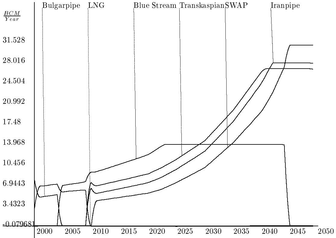
Figure 20: Case A, Scenario 6: Supply by competitive pipelines under optimization of “Transcaspian” maximal capacity.
