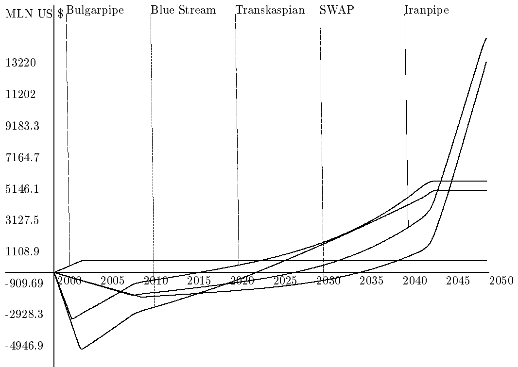
Figure 10: Case A, Scenario 1: Net present values of gas pipeline projects.
