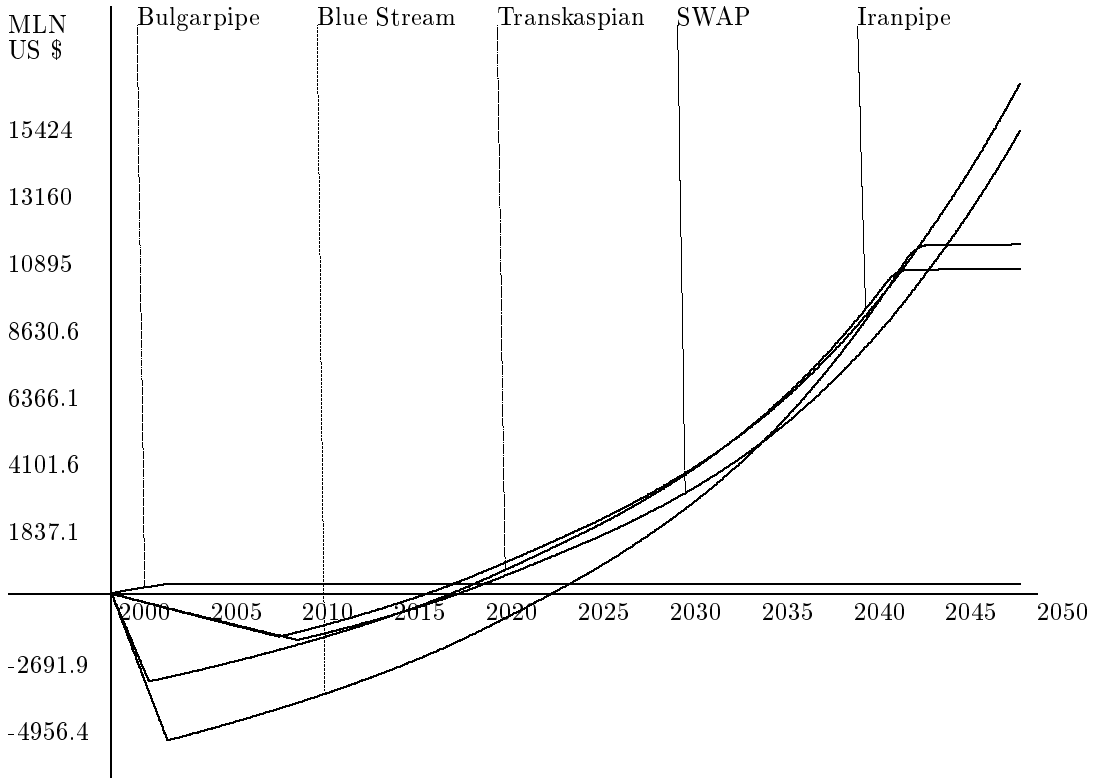
Figure 23: Case B, Scenario 1: Net present values of gas suppliers.
