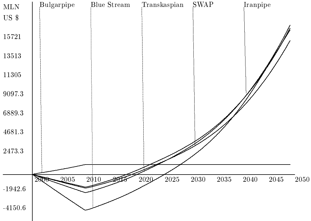
Figure 25: Case B, Scenario 3: Net present values of competitors.
