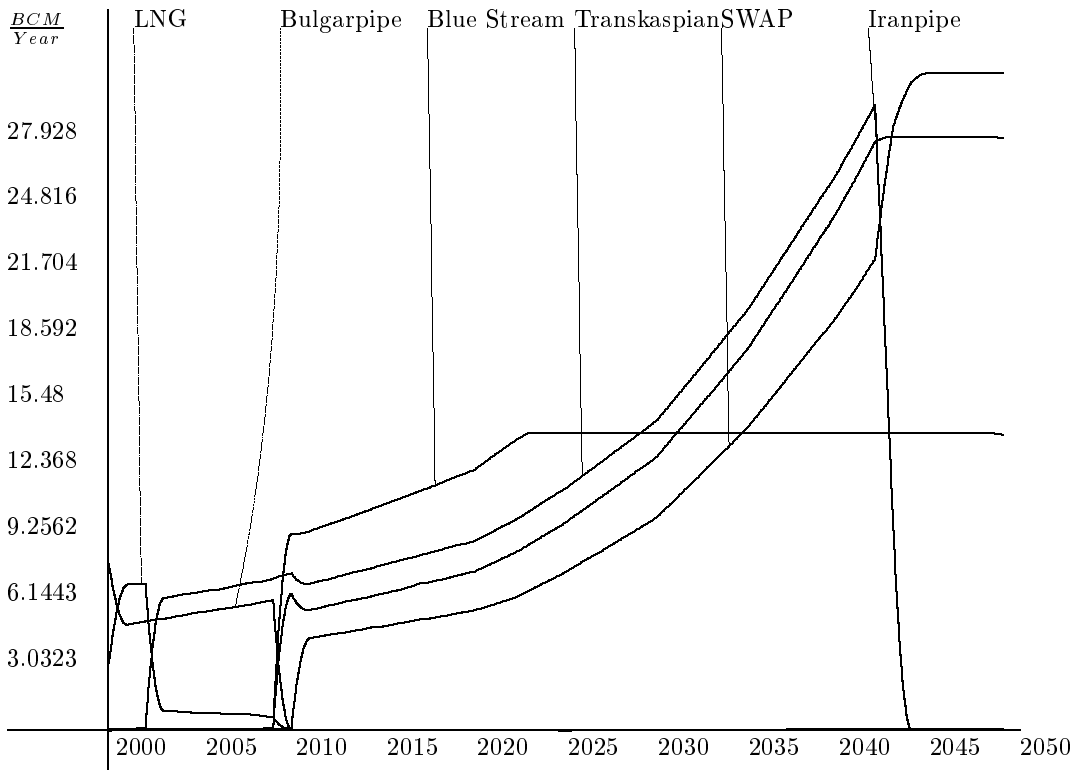
Figure 13: Case A, Scenario 2: Gas deliveries if construction of “Blue Stream” is completed in 2009.
