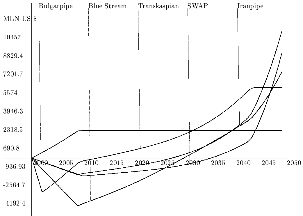
Figure 14: Case A, Scenario 2: Net present values of gas suppliers if construction of “Blue Stream” is completed in 2009.
