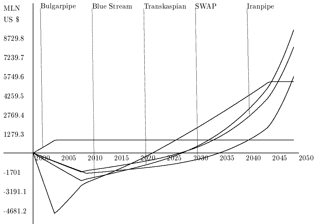
Figure 17: Case A, Scenario 4: Net present values of gas suppliers in the game scenario.
