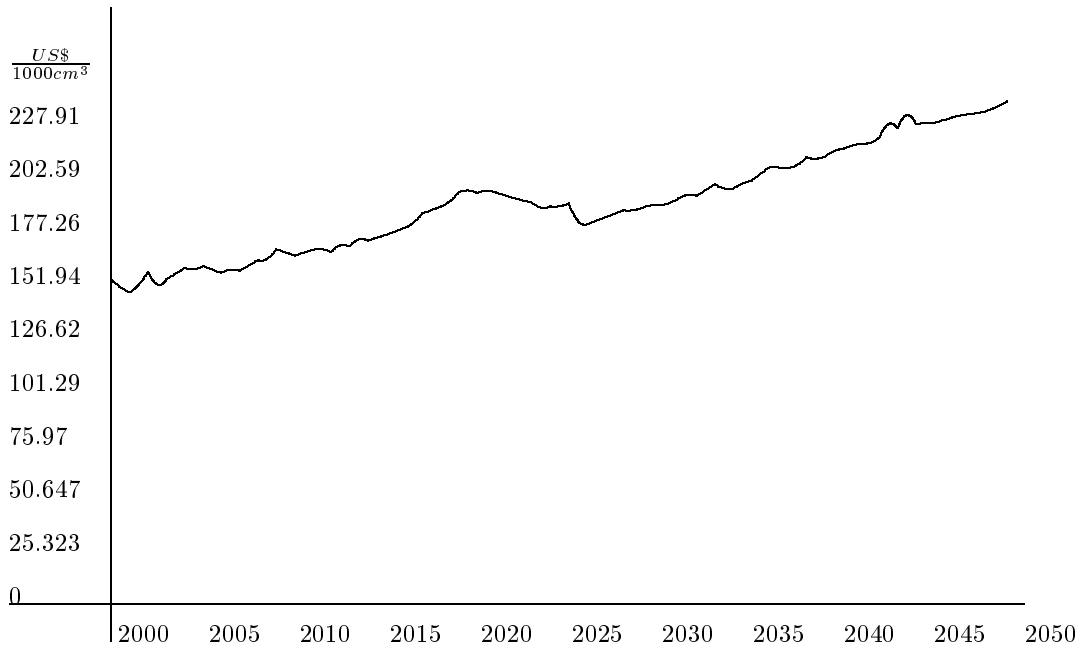
Figure 21: Case B, Scenario 1: Dynamics of gas price.
