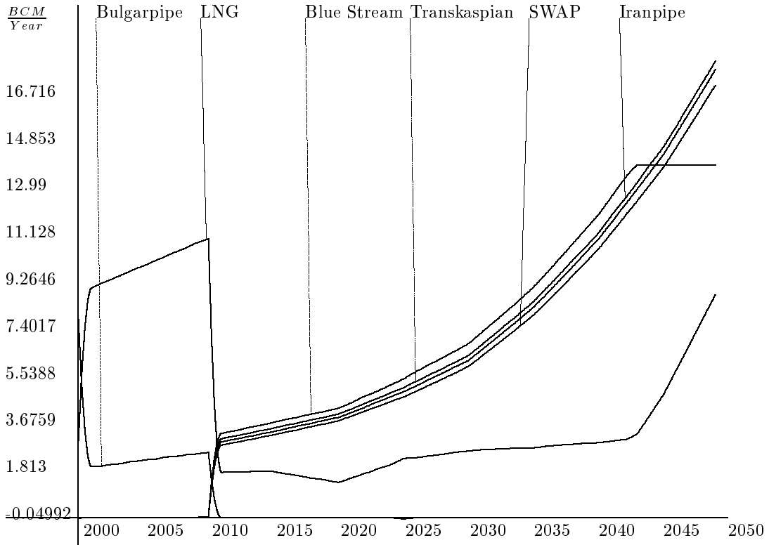
Figure 24: Case B, Scenario 4: Supply by competitive pipelines.
