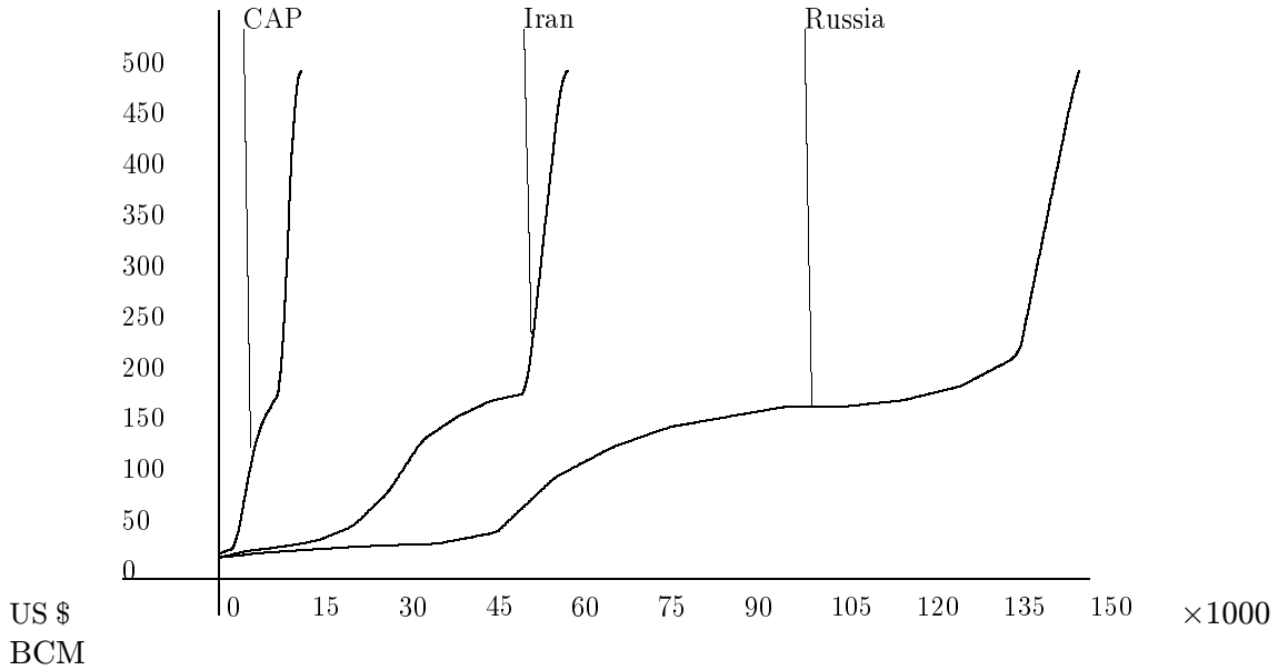
Figure 1: Cumulative gas supply cost curves.
