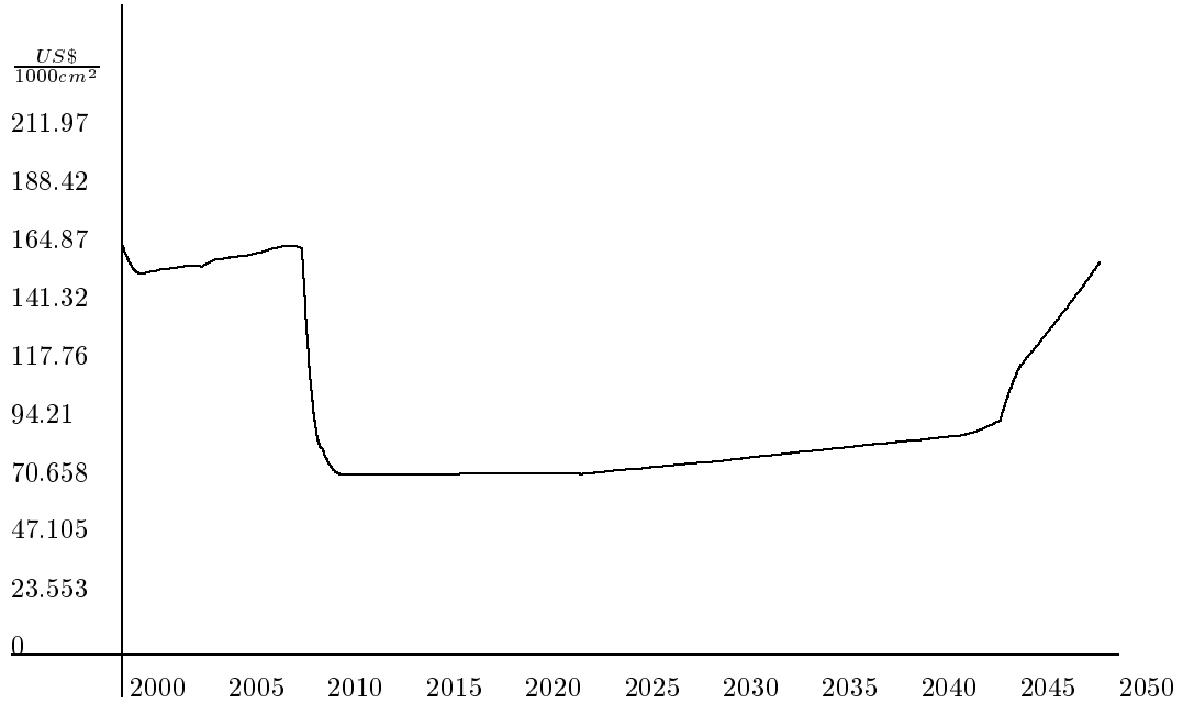
Figure 18: Case A, Scenario 4: Dynamics of gas price in the game scenario.
