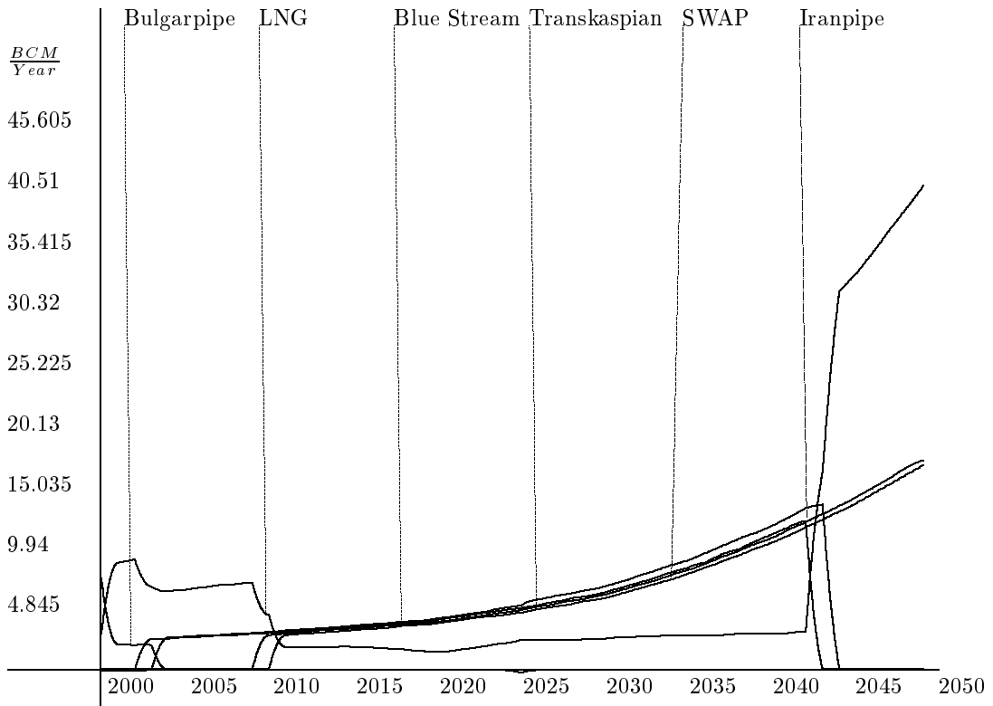
Figure 22: Case B, Scenario 1: Gas supply.
