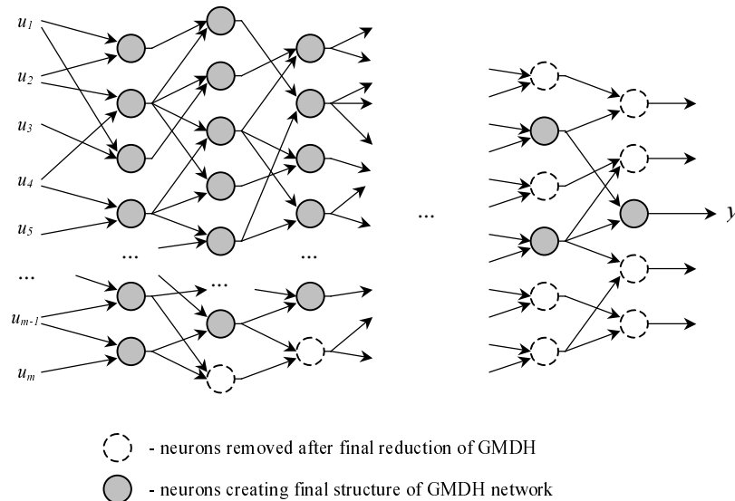
Fig. 7. Final reduction of not used neuron of the GMDH type
