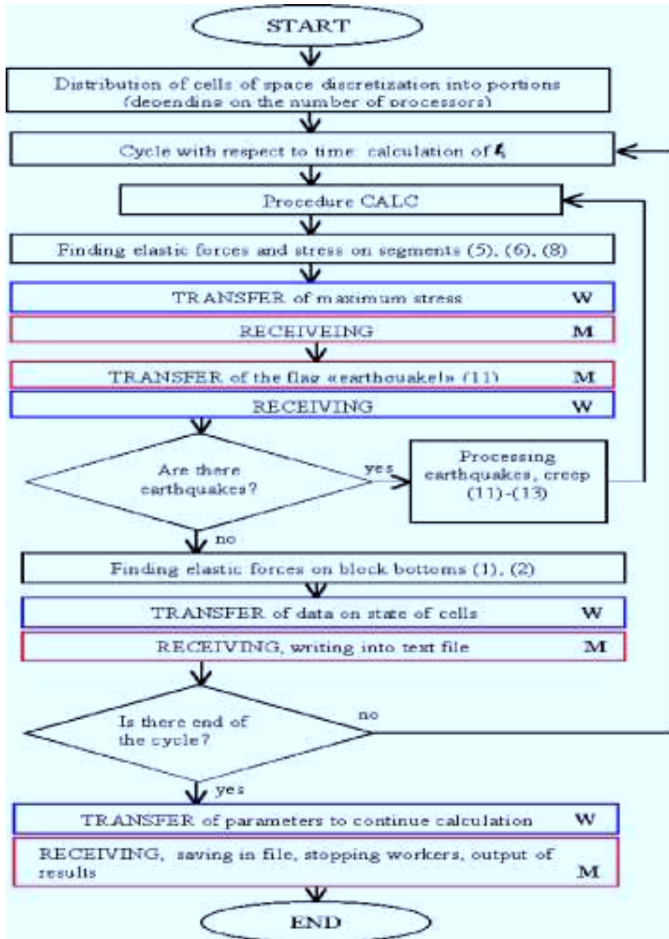
Fig. 3. Procedure RUN
