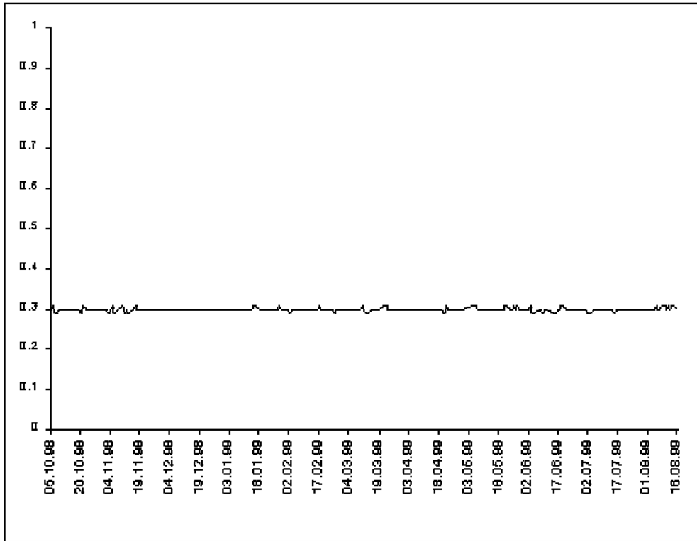
Fig.2. Portfolio risk (1)
