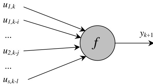
Fig. 13. The structure of the GMDH neuron defined for the dynamic discrete systems
