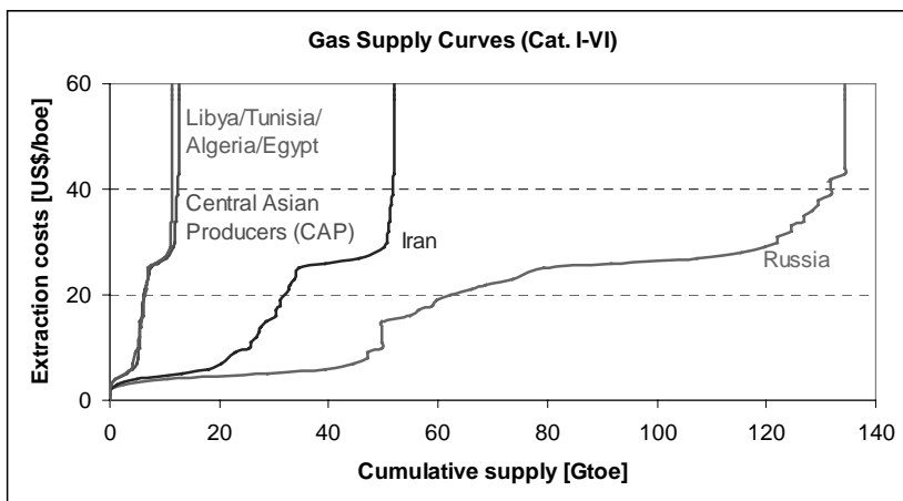
Fig. 4-2. Cumulative gas supply cost curves (Natural Gas Cat. I-VI, based on Rogner method and regional data, adapted by Roehrl).
