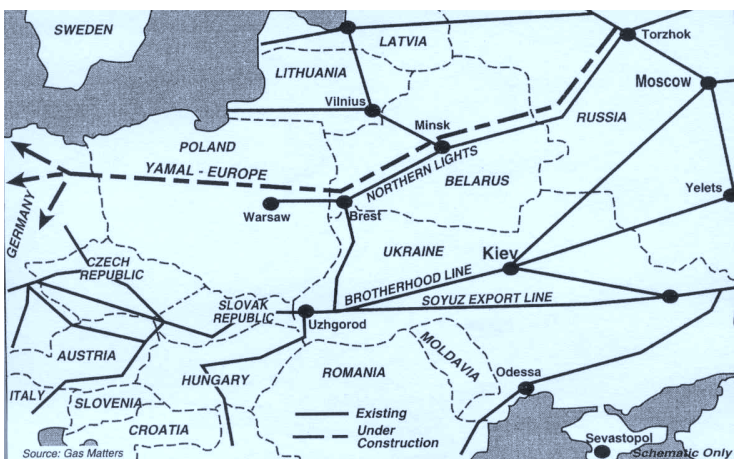
Fig. 6-2. Main export pipelines from the countries of the Former Soviet Union (FSU) to Western and Eastern Europe. Source: Gas Matters.
