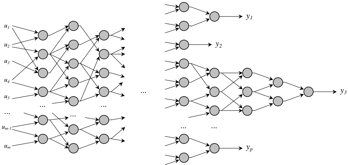
Fig. 12. The structure of the GMDH multi-output network constructed by the method of the multi criteria selection
