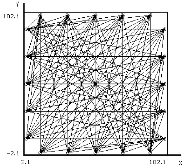
Fig. 2: The set of seismic rays under testing.
