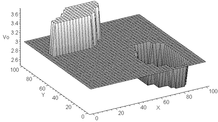
Fig. 3: Model distribution v_0(x,y) of seismic signal propagation velocity as a function of spatial coordinates.
