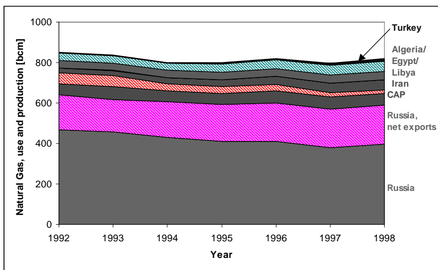
Fig. 5-1. Natural gas use and production in the 1990s. The difference between production and use is the net exports.
