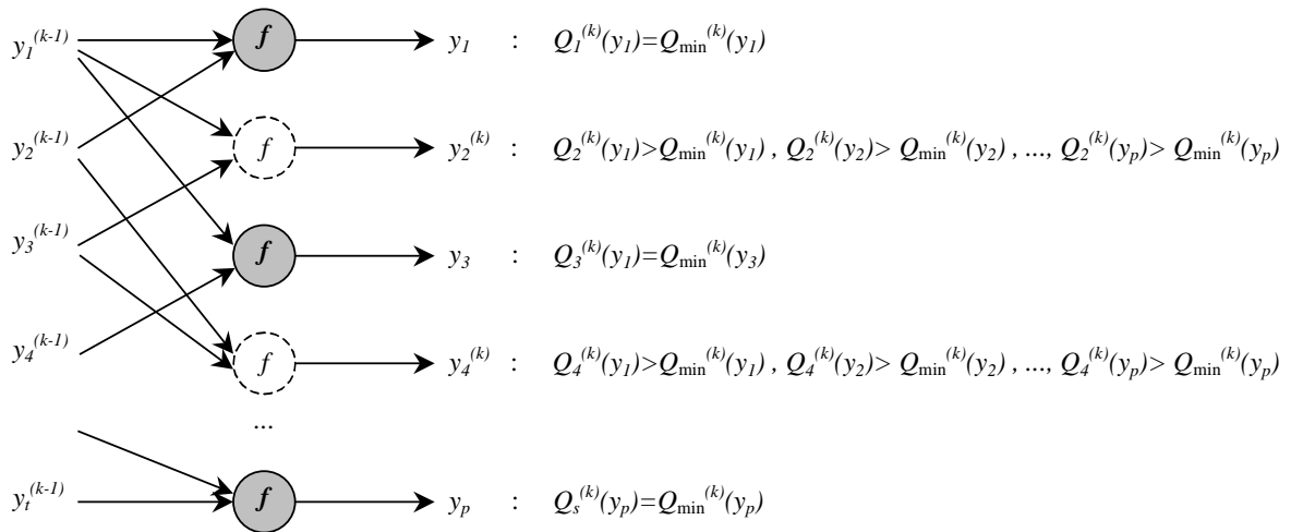
Fig. 9. Scheme of the classification of the output neuron of the GMDH network
