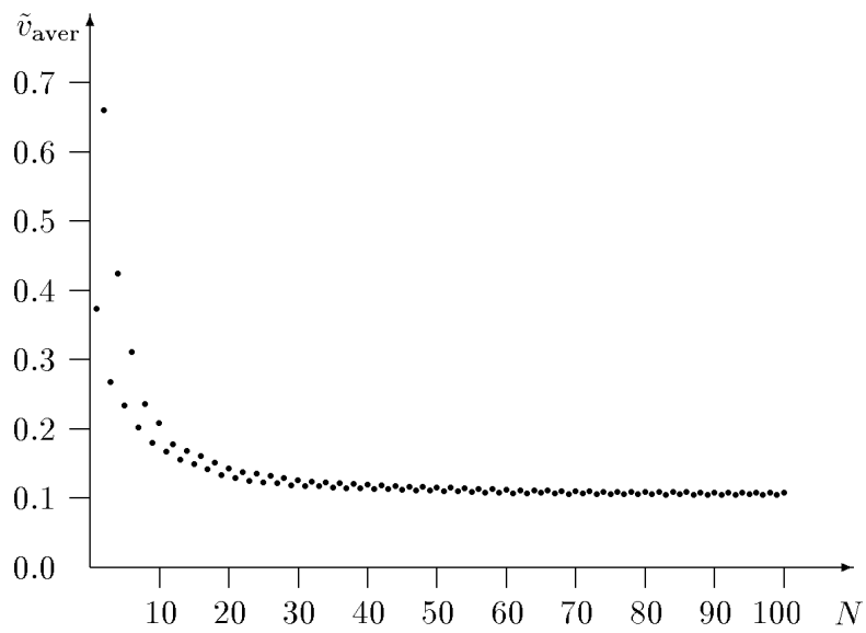
Fig. 6: Dependence of average error of velocity reconstruction on number of iterations N .
