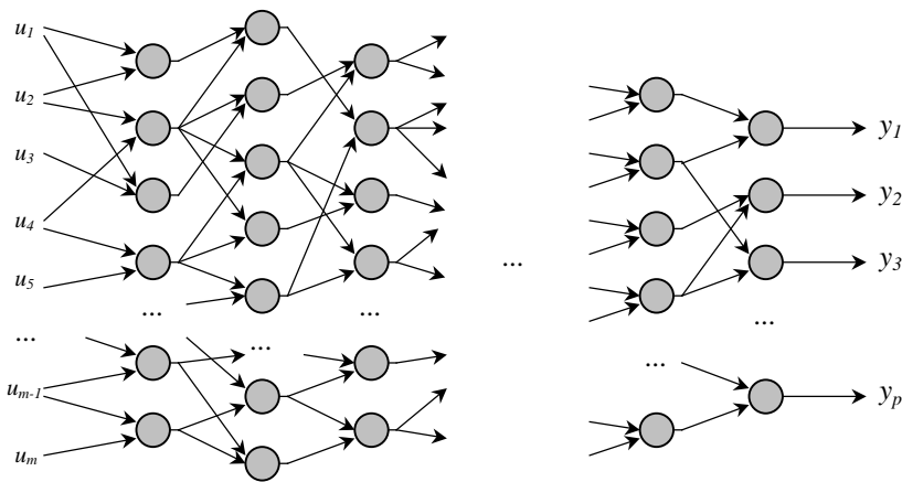
Fig. 10. The multi-output network of the GMDH type structure
