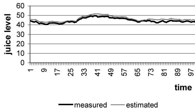
Fig. 18. The course of the variability of the measured juice level and adequate estimated values. The experiments run for the sugar processes confirm the capabilities of the GMDH network to model accurately both the values of the measured signals and trends of their changes in case of the dynamic systems also.
