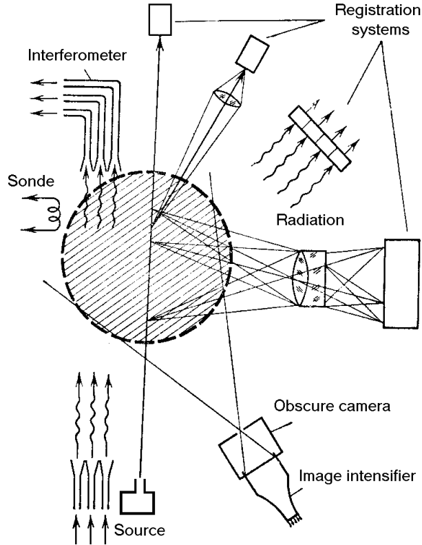
Fig. 1: Scheme of diagnostics of high-temperature plasma [17].
