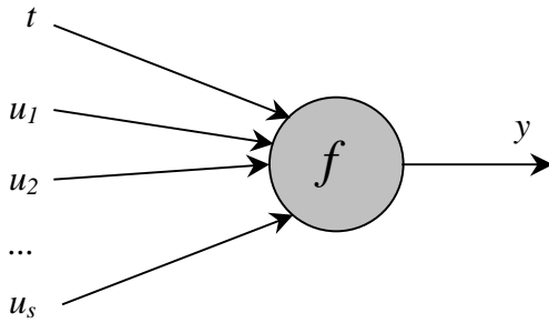
Fig. 14. The structure of the dynamic GMDH neuron synchronized by the parameter of time
