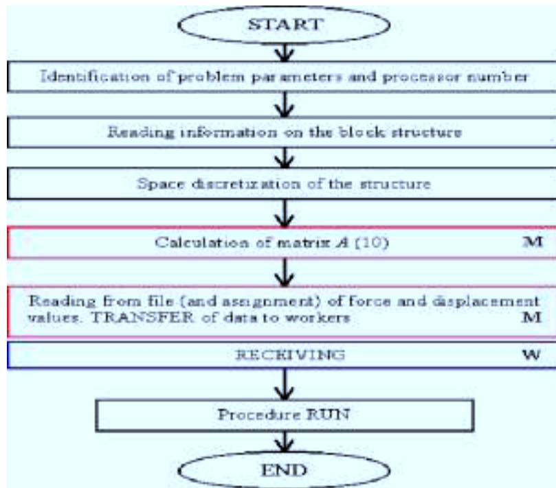
Fig. 2. Scheme of parallelization of the block model. Notation: operations carried out only by master are marked by «M», only by workers – by «W».
