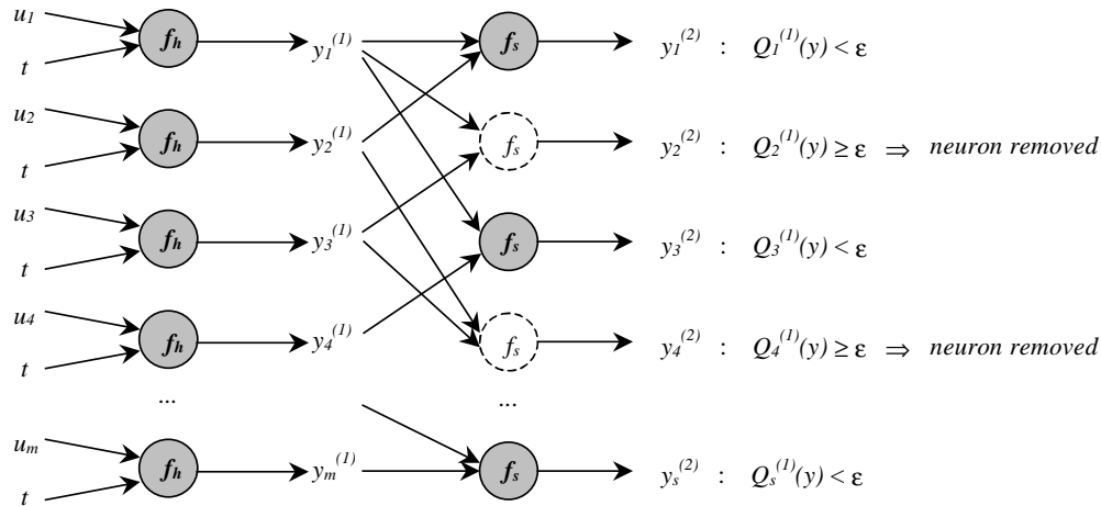
Fig. 15. Synthesis process and selection of the neurons in the GMDH harmonic network
