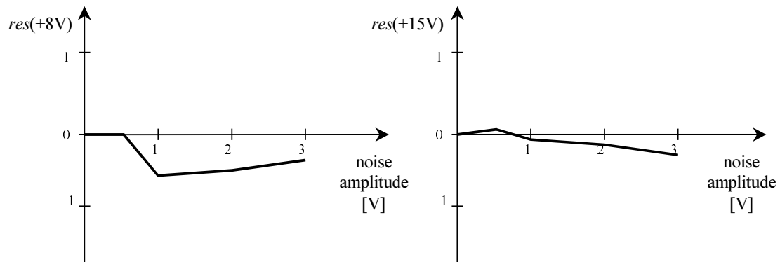
Fig. 17. The charts of variability of the selected residues and their dependence on the level of the measuring noises
