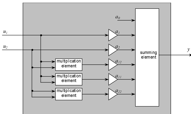
Fig.1. An example of a scheme of hardware realization of the GMDH elementary polynomial function
