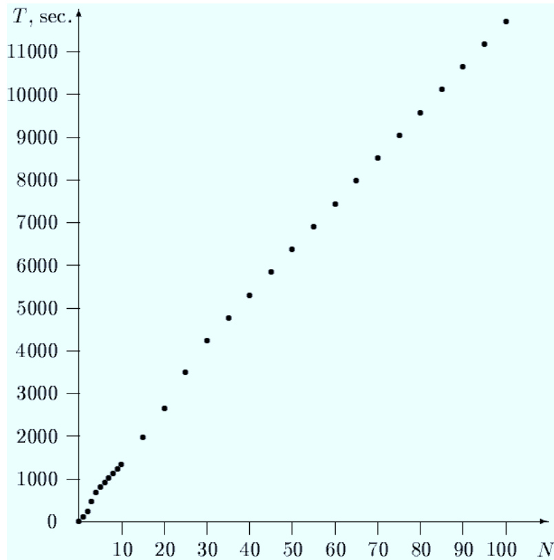
Fig. 7: Dependence of computation time on number of iterations N .
