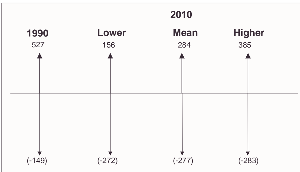
Figure 17. Net fluxes, in Tg C.
