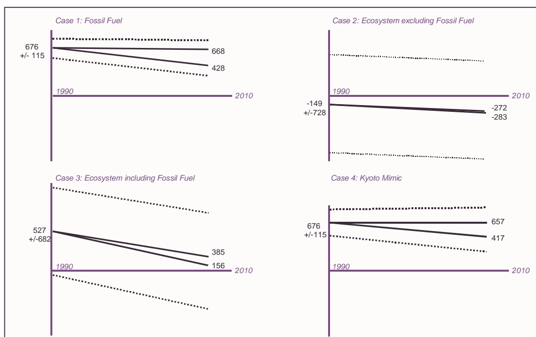
Figure 19. Changes in total flux balances (solid lines) and uncertainty ranges (dotted lines) for the Kyoto Protocol commitment period (1990–2010), in Tg C.
