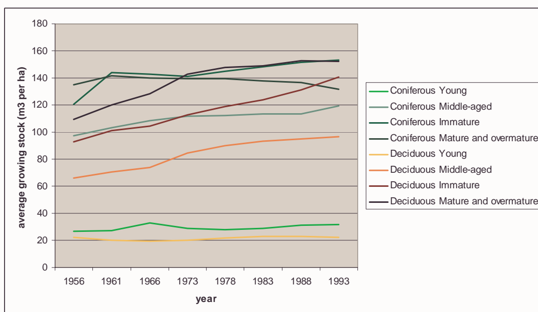
Figure 15. Dynamics of average growing stock of Russian forests (1956–1993), in m 3 /ha.
