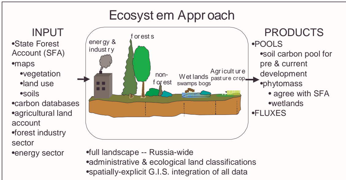
Figure 3. Ecosystem approach used in the Russian FCA.
