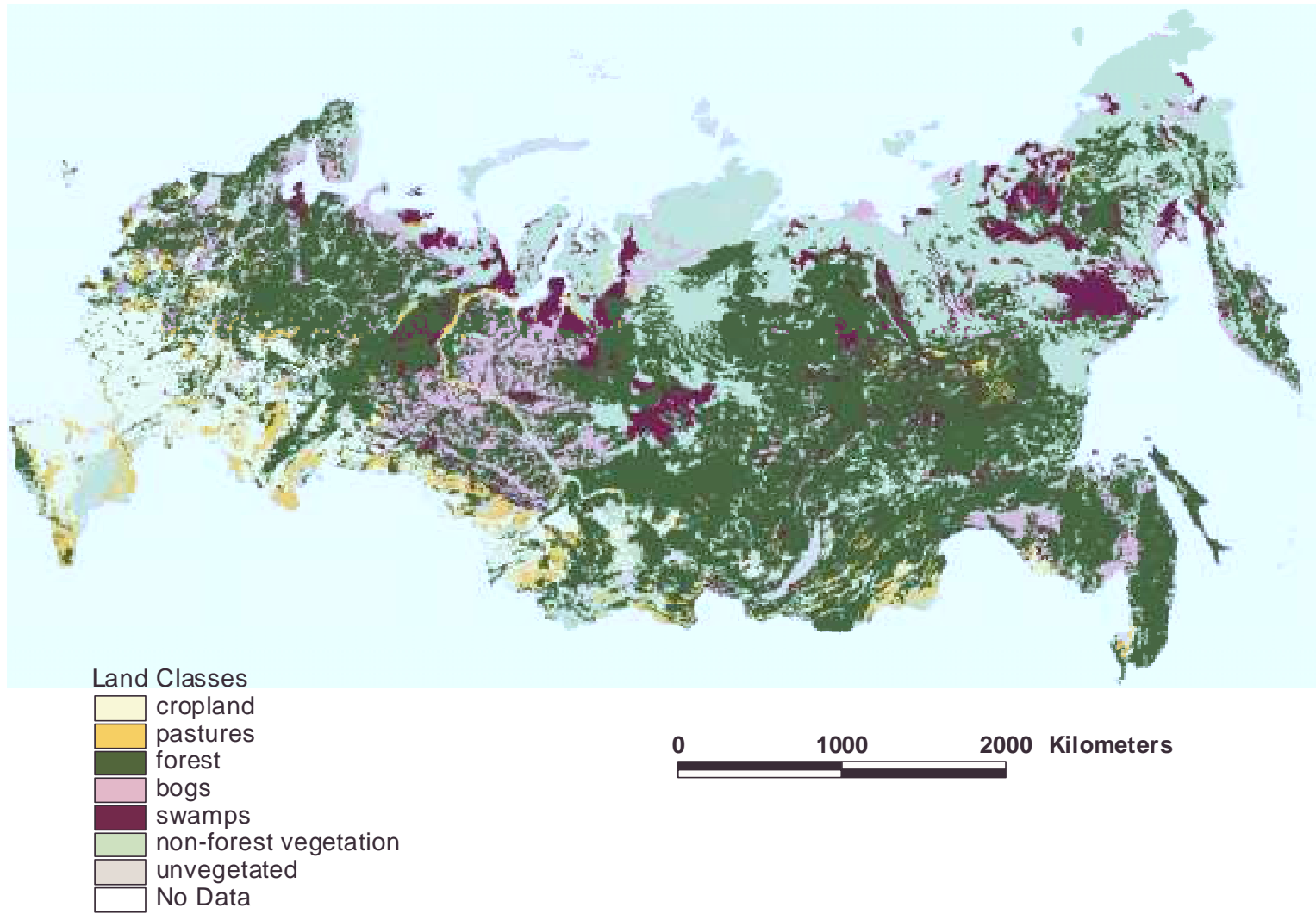
Figure 11. Land class map (LCM).
