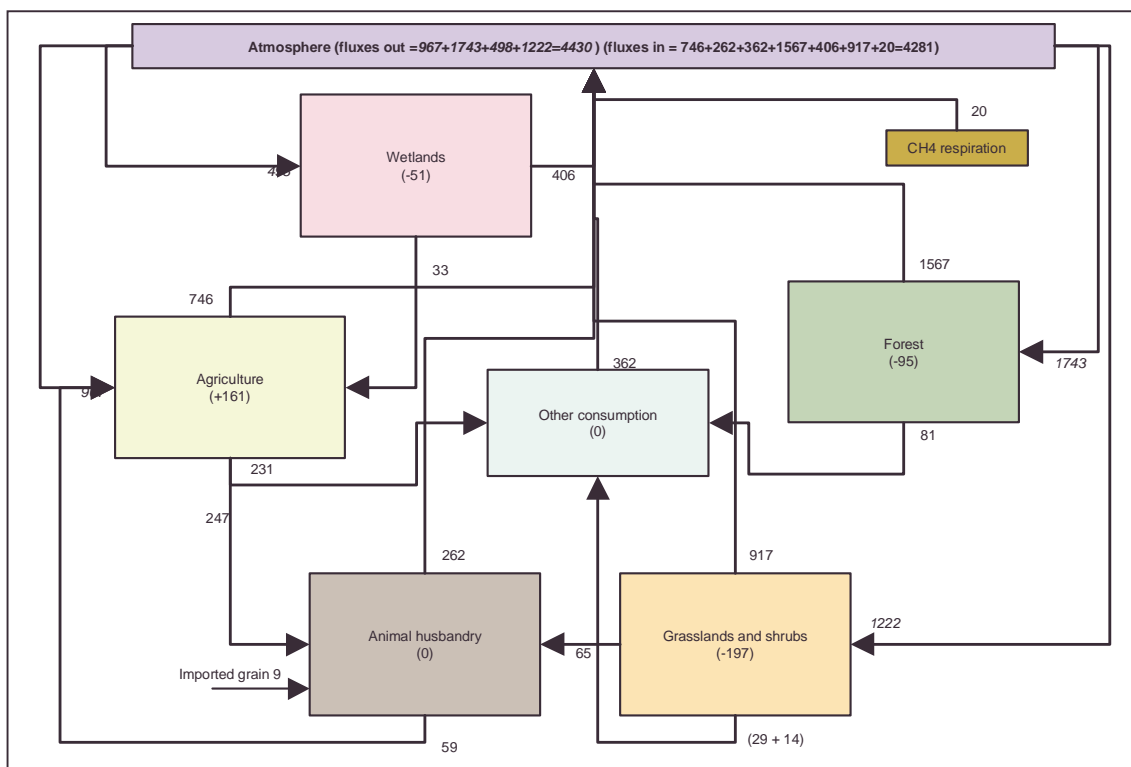
Figure 13. Fluxes between atmosphere and terrestrial ecosystems (1990).
