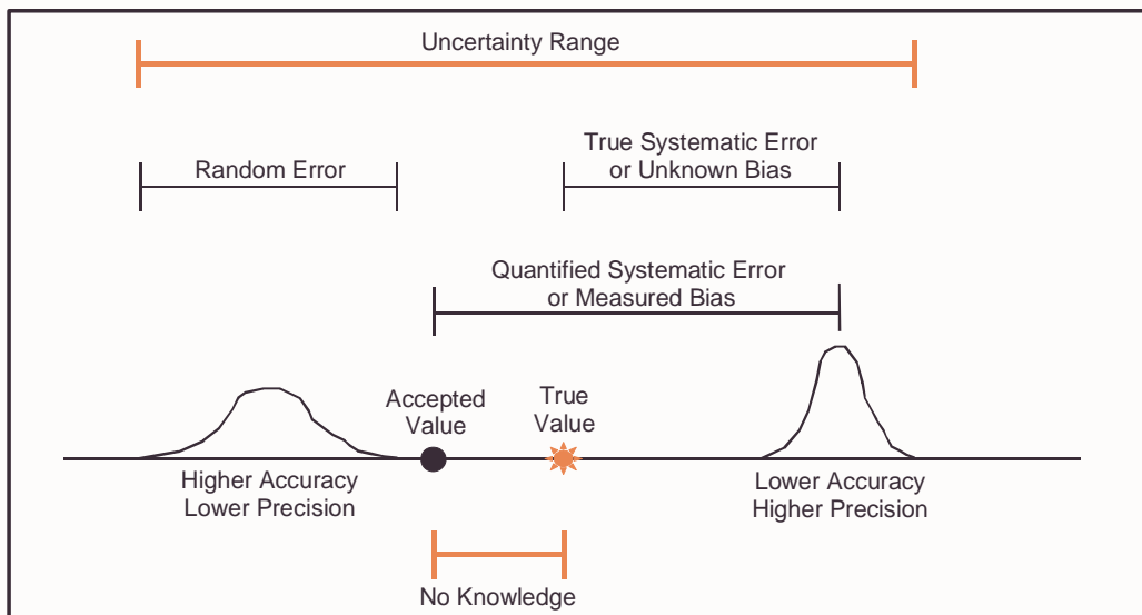
Figure 12. A hypothetical uncertainty range for two sets of measurements of the same phenomenon (individual variable).
