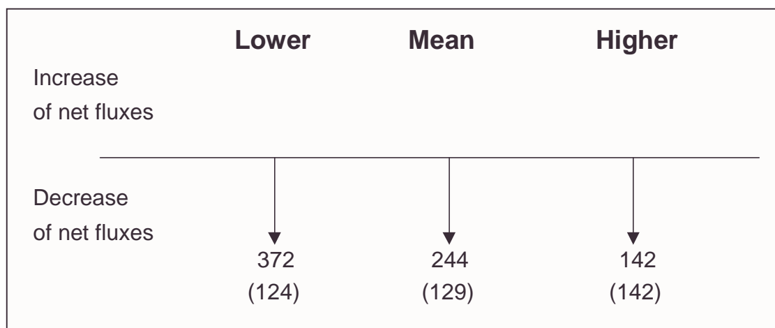
Figure 18. Changes of the net fluxes (1990–2010), in Tg C.
