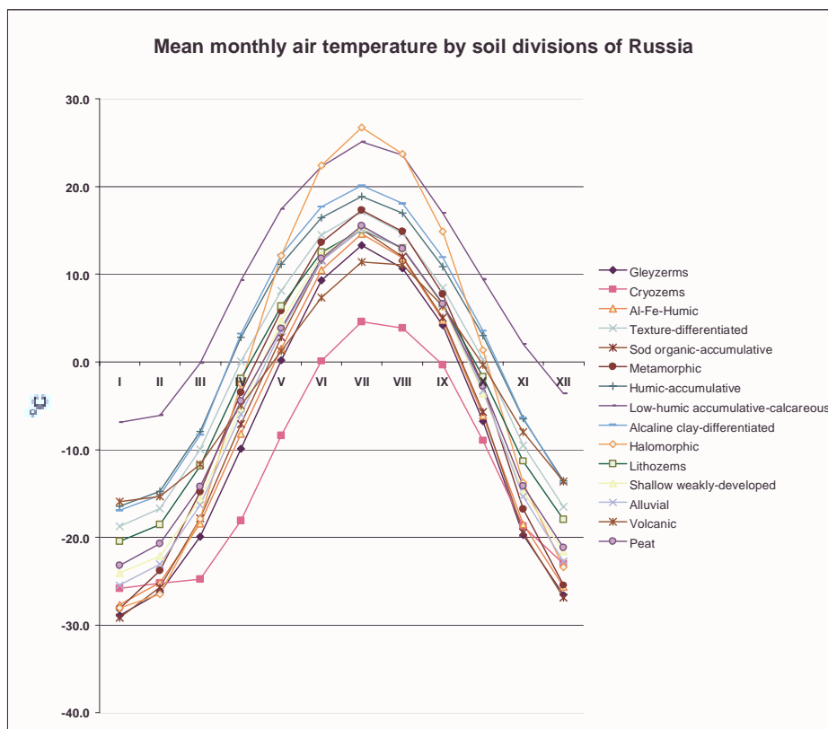
Text Box T.7 Aggregated, area-weighted mean monthly temperature by soil divisions of Russia: estimate of the period of time with temperature > 0° C.
