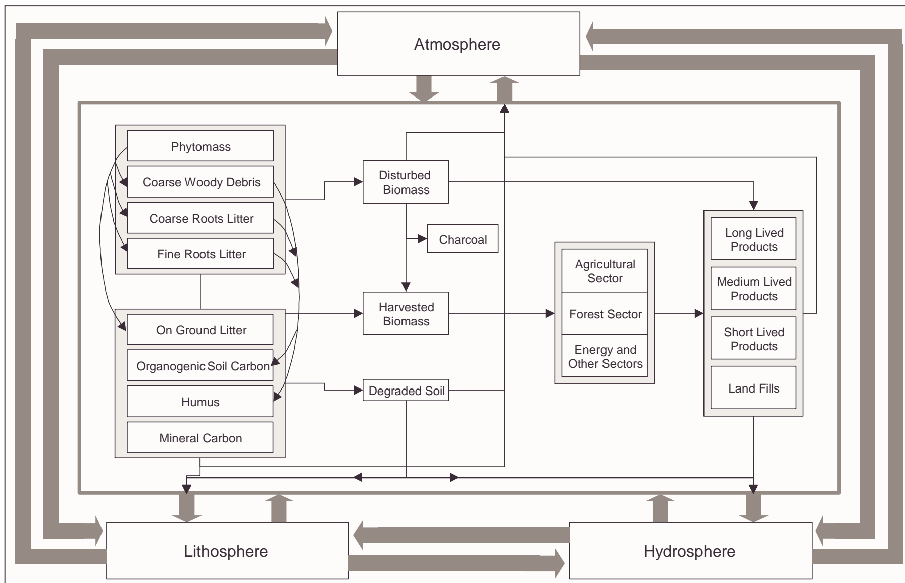
Figure 2. Pools and fluxes considered in the Russian FCA.
