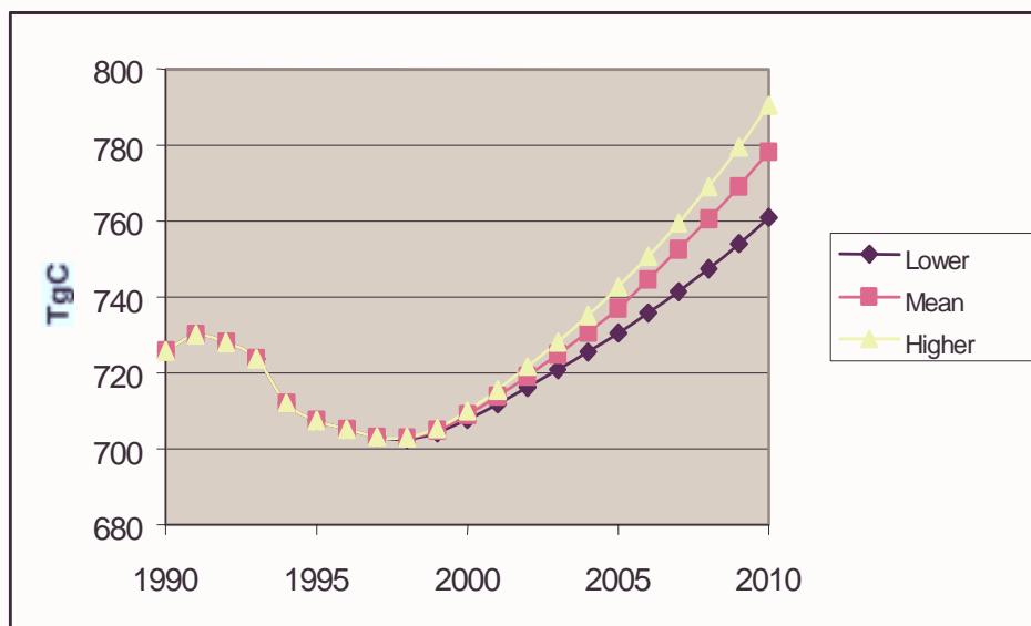
Figure 16. Carbon Pools of the Forest Products Sector Over Time, in Tg C.
