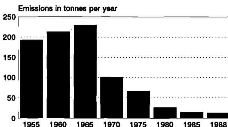
Figure 2.1. Atmospheric Cadmium Emissions - Northrhine-Westfalia
