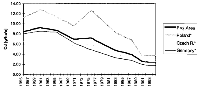
Fig. 4 Average atmospheric cadmium deposition during 1955 and 1994
