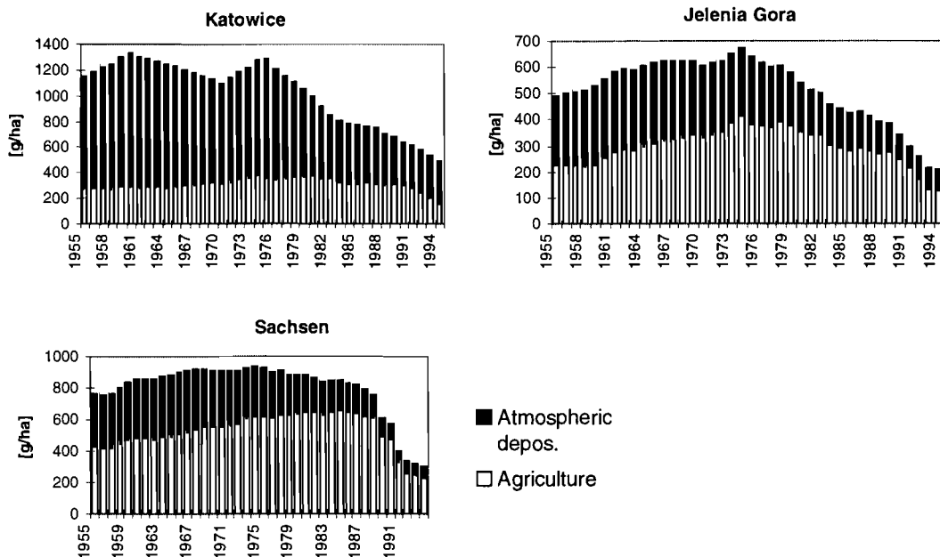
Fig 8. Atmospheric and agricultural Zinc load to agricultural soils for three provinces in the project area
