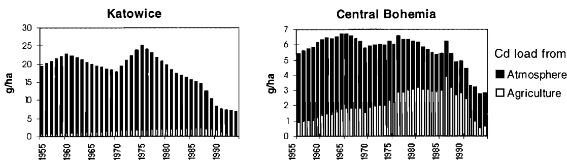
Fig. 6. Total cadmium load to agricultural land for two districts in the project area
