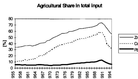
Fig. 9 Agricultural Share in total load of Zn, Cd and Pb based on average values for the project area
