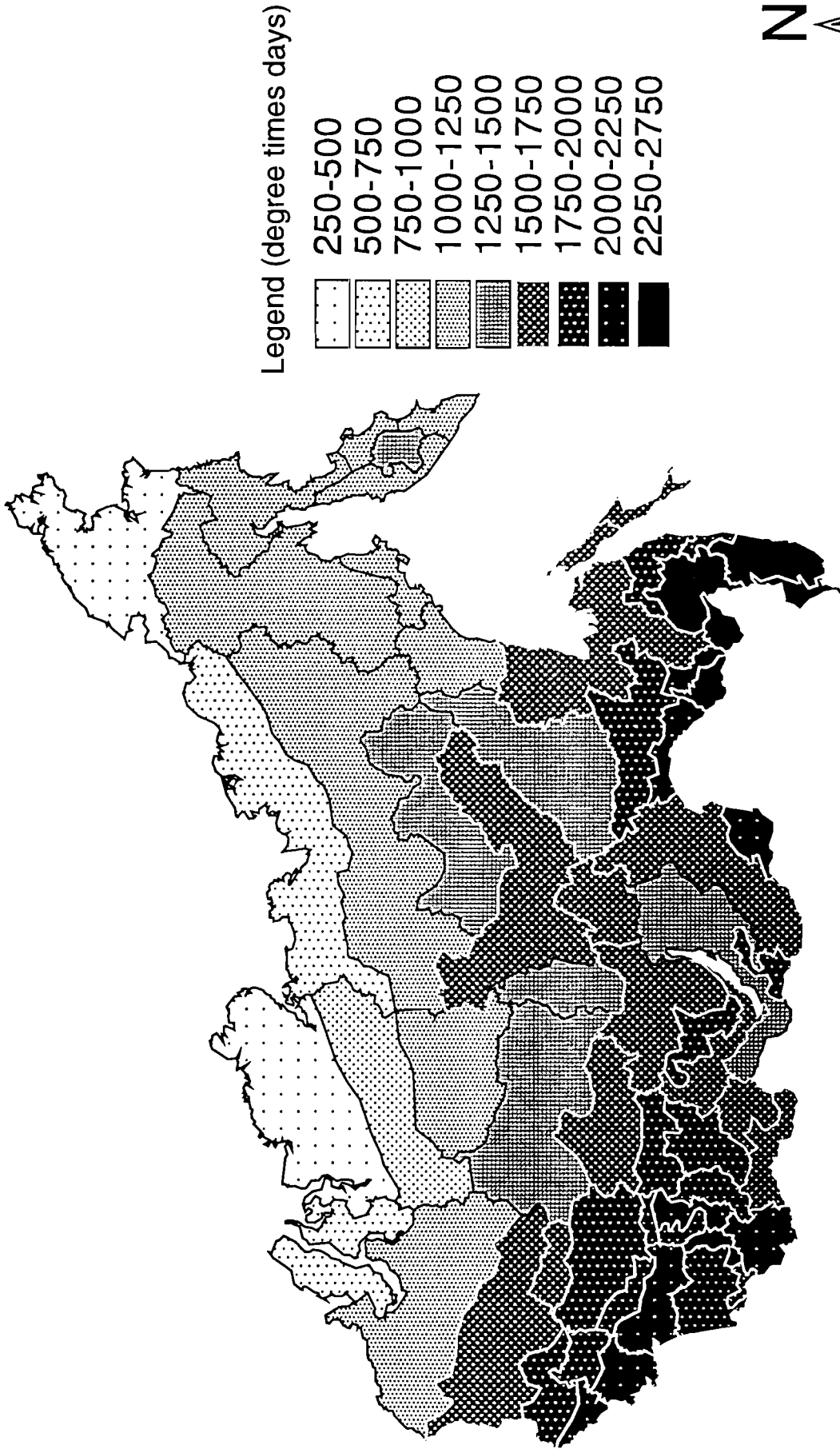
Map 4.5. Degree times days with an average temperature > 5° C.
