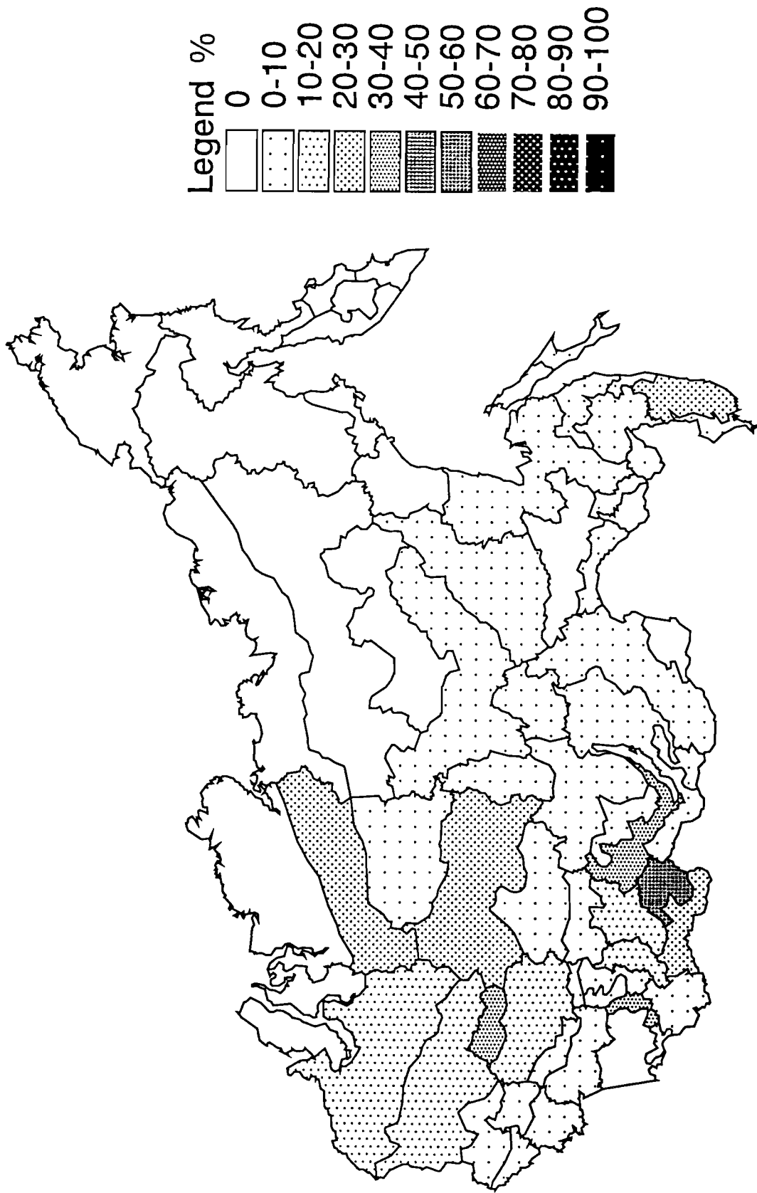
Map 7.6. Percentage of Forested Areas dominated by cedar.
