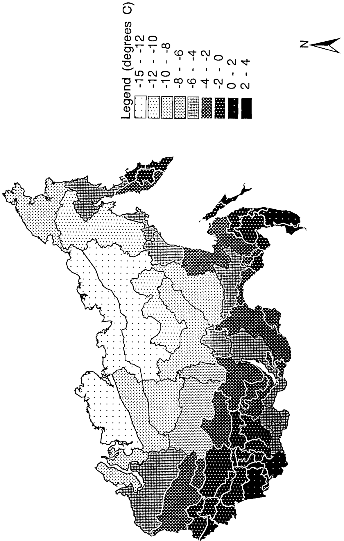
Map 4.2. Average annual air temperature.
