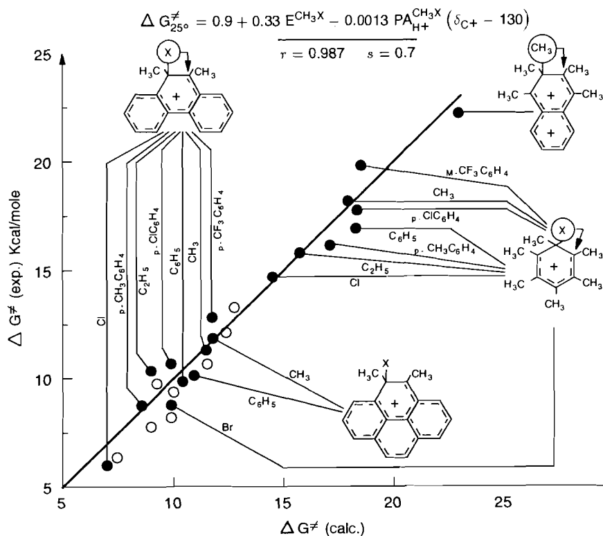
Figure 3. Correlation of calculated and experimental free energies of methyl 1,2-shifts for various arenonium ions.
