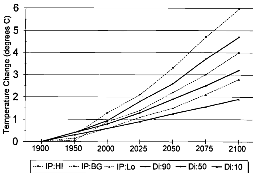
Figure 7. Projected temperature change (IPCC and DICE model).
