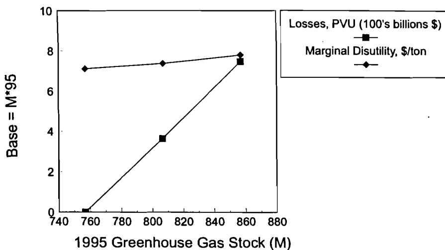
Figure 6. Marginal and total disutility as function of CO 2 stock.
