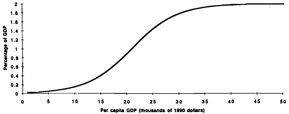
Figure 5. Willingness-to-pay to avoid 2.5°C change in temperature: non-market (ecological) damages.
