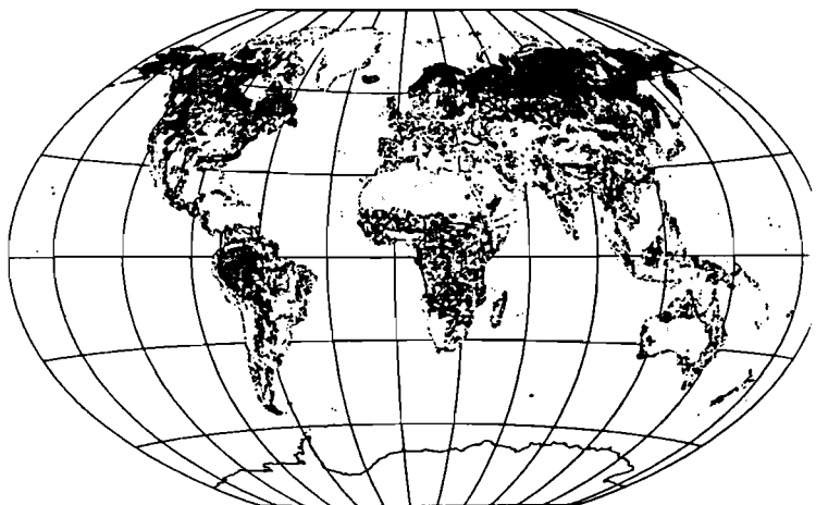
Net Carbon Flux 2050 Conventional Wisdom (ton C/km 2 )
