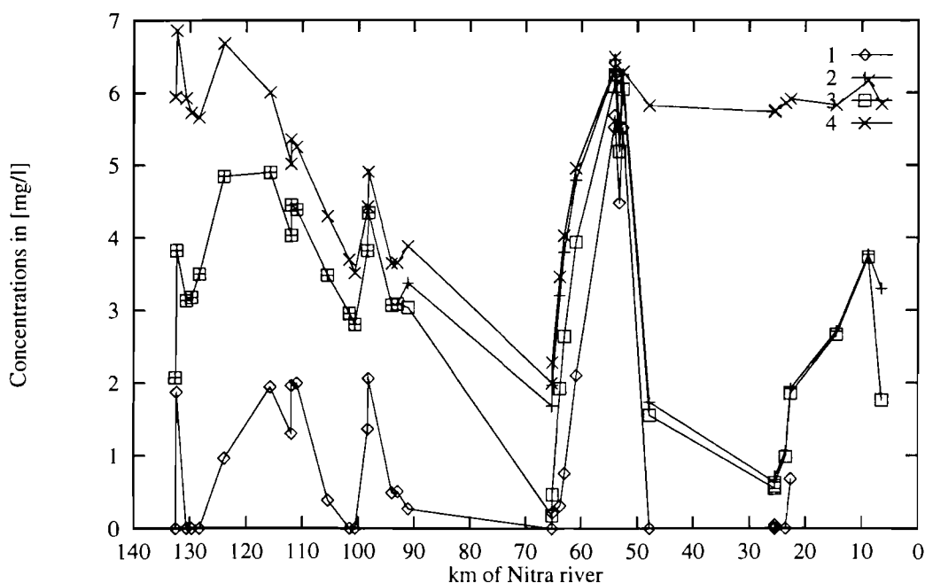
Figure 4: DO concentrations for 4 scenarios.
