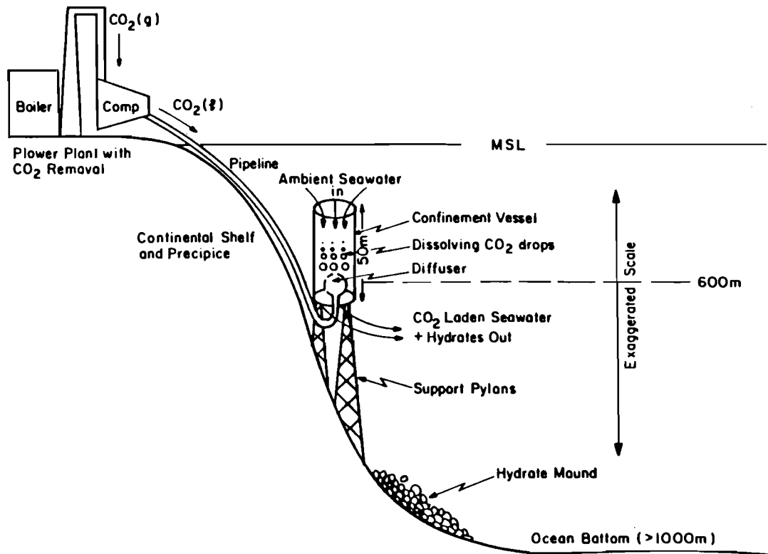
Figure 21. Scheme of CO 2 release system with confinement vessel suggested for deep ocean disposal of sequestered CO 2 . Source: Golomb.
