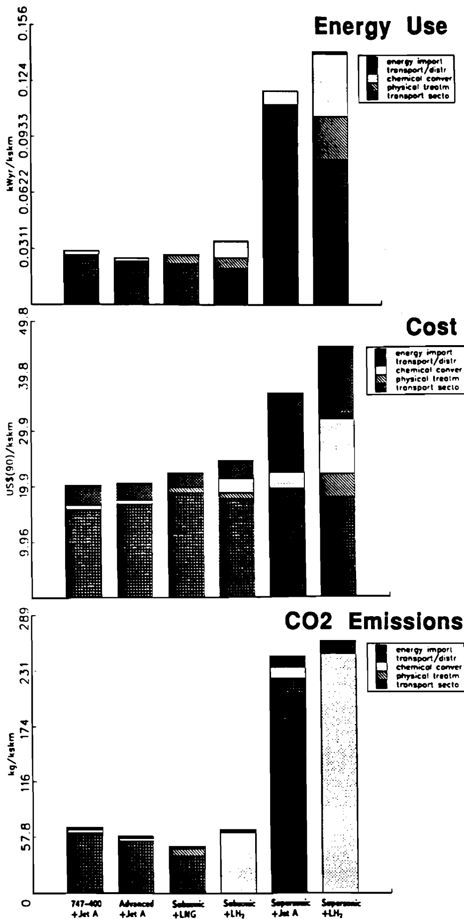
Fig. 6. Energy requirements, costs and CO 2 emissions for six energy chains ending with air passenger transport. Aircraft include a Boeing 747-400 (Jet A), an advanced (Jet A), a liquid methane (LNG) and liquid hydrogen (LH 2 ) wide-body transports; a Jet A and liquid hydrogen supersonic transports. Liquefied hydrogen is produced from natural gas.
