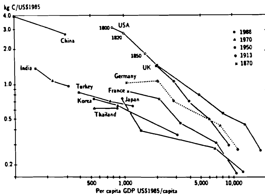
Fig. 1. Energy CO 2 emissions intensity per constant GDP, in kg carbon per constant 1985 US$ versus per capita GDP in constant 1985 US$ (Grübler and Fujii, 1991).
