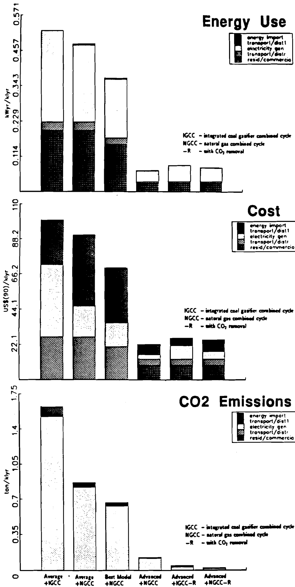
Fig. 5. Energy requirements, costs and CO 2 emissions for six energy chains ending with refrigeration. Average, best new and advanced refrigerators (200 liters) are considered and two different power plans: An IGCC and NGCC and IGCC-R and NGCC-R with CO 2 recovery.
