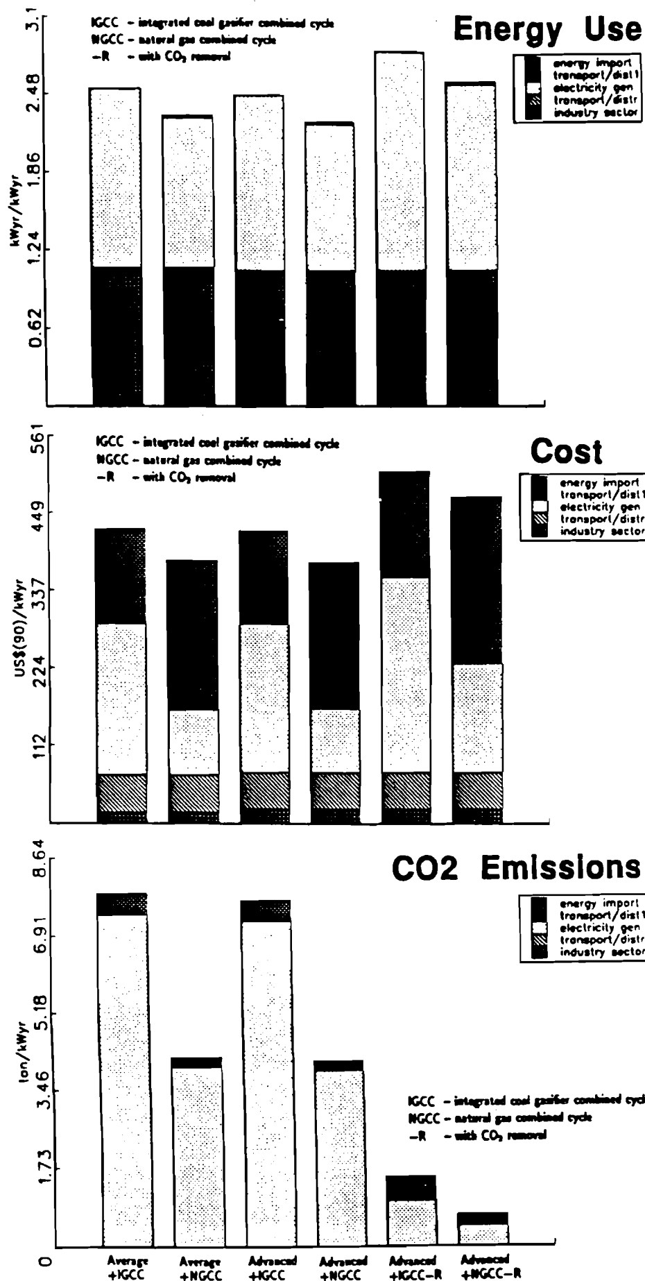
Fig. 4. Energy requirements, costs and CO 2 emissions for six energy chains ending with industrial motor drives. Average and advanced motors (112 kW) are considered and two different power plans: An IGCC and NGCC and IGCC-R and NGCC-R with CO 2 recovery.
