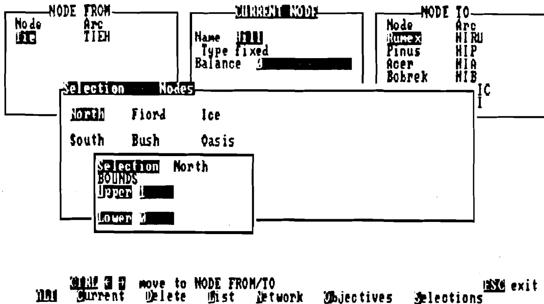
Figure 18: BOUNDS window
