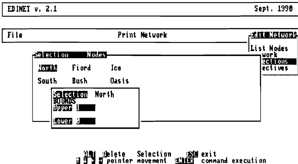
Figure 7: OBJECTIVES window
